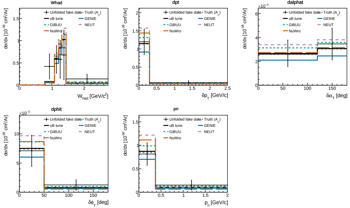
Figure 25: Proton-tagged ( CC1mu1pi1p ) released differential cross sections for FHC: the calorimetric hadronic mass W_{\text{had}} and the four transverse-kinematic-imbalance observables \delta p_T , \delta \alpha_T , \delta \phi_T and p_n (the withdrawn W_{\pi p} shape is not shown; see the technical supplement). Unfolded fake data (black points) are compared to the A_C -smearred fake-data truth (grey dashed), the MicroBooNE tune (black), and the GENIE (blue), GiBUU (green), NEUT (purple) and NuWro (orange) predictions built for the same proton-tagged phase space. \delta \alpha_T rises toward 180^\circ , the signature of final-state interactions.
