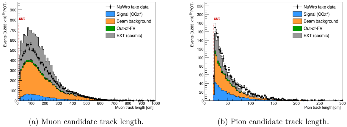
Figure 3: N–1 track-length distributions. Muon threshold: > 10 cm (Cut 4); pion threshold: > 20 cm (Cut 5).
