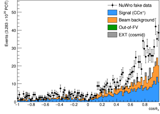
(b) Pion \cos \theta .
