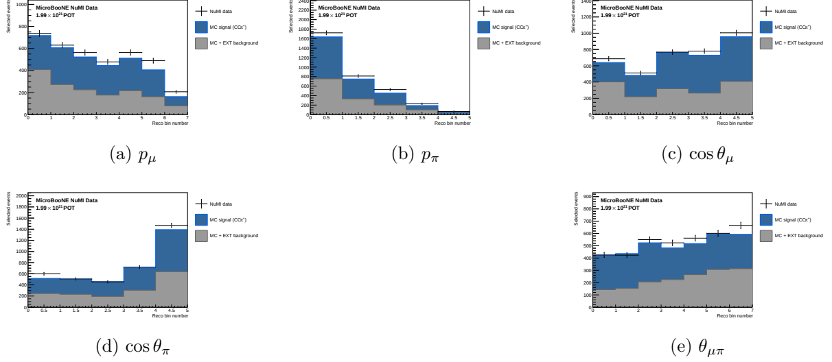
Figure 11: Reconstructed-space spectra, combined FHC+RHC (per-mode normalised); same components as Fig. ??.
