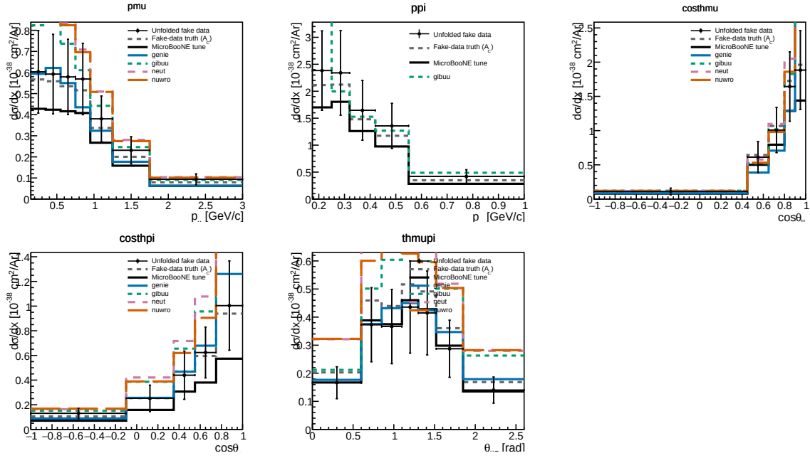
Figure 17: Combined FHC+RHC ( \nu_\mu + \bar{\nu}_\mu ) differential cross sections on the current per-mode-normalised fake data, with the fluence-weighted combined generator predictions.
