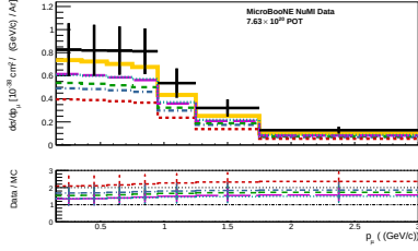
(a) d\sigma/dp_\mu (framework, optimised binning).
