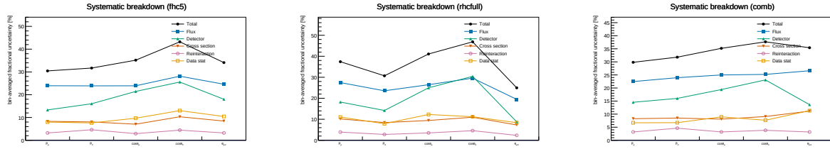
Figure 18: Bin-averaged fractional systematic uncertainty by source vs. observable, for FHC (left), RHC (centre) and combined (right) — the figure form of Tables ??–??. Colours use the Okabe-Ito colourblind-safe palette with distinct markers per source: total (black), flux (blue), detector (green), cross section (vermillion), reinteraction (purple), data stat (orange).
