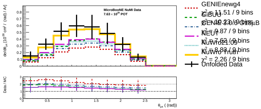
Figure 5: Unfolded d\sigma/d\theta_{\mu\pi} .
