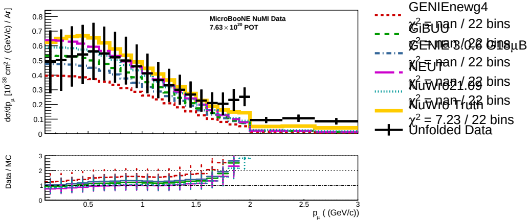
Figure 2: Unfolded d\sigma/dp_\mu .
