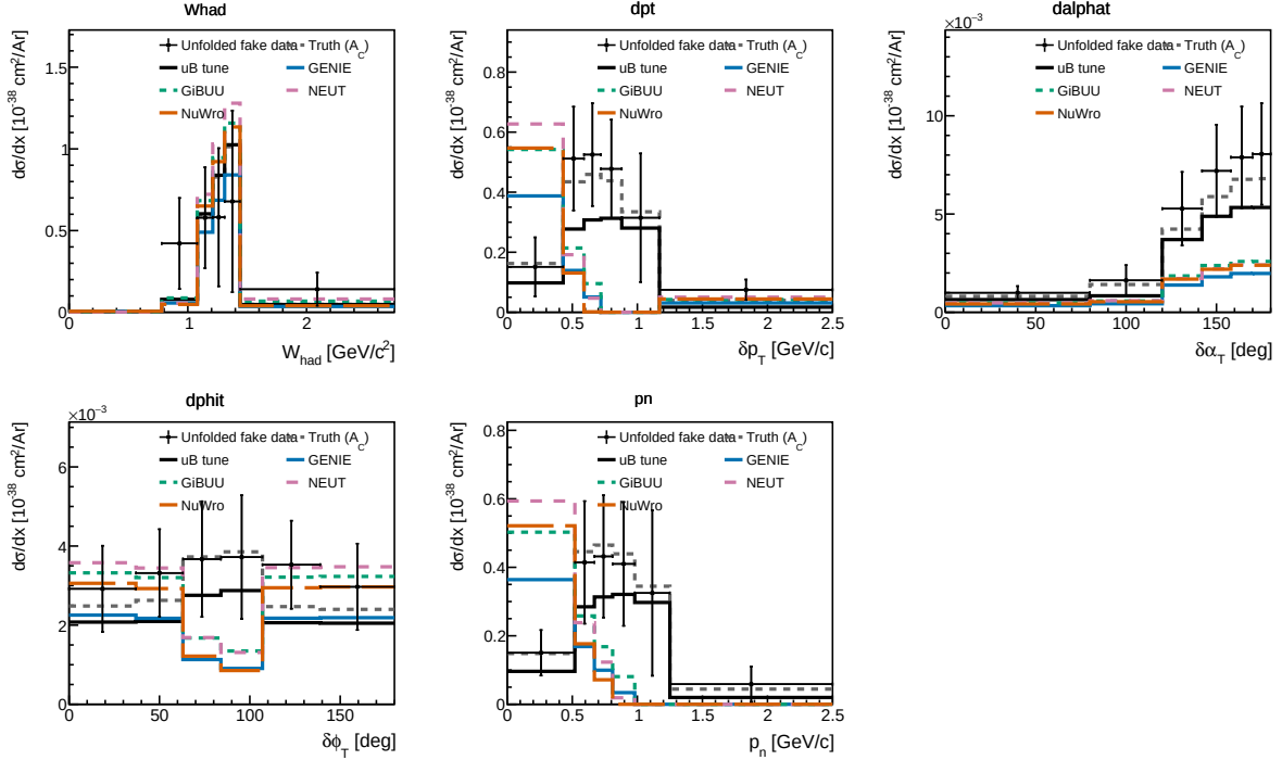
Figure 24: Proton-tagged ( \text{CC1}\mu\text{1p1p} ) released differential cross sections for FHC: the calorimetric hadronic mass W_{\text{had}} and the four transverse-kinematic-imbalance observables \delta p_T , \delta\alpha_T , \delta\phi_T and p_n (the withdrawn W_{\pi p} shape is not shown; see the technical supplement). Unfolded fake data (black points) are compared to the A_C -smearred fake-data truth (grey dashed), the MicroBooNE tune (black), and the GENIE (blue), GiBUU (green), NEUT (purple) and NuWro (orange) predictions built for the same proton-tagged phase space. \delta\alpha_T rises toward 180^\circ , the signature of final-state interactions.
