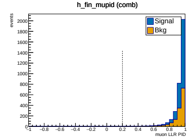
(c) Muon LLR PID, comb.
