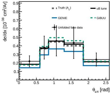
thmupi
