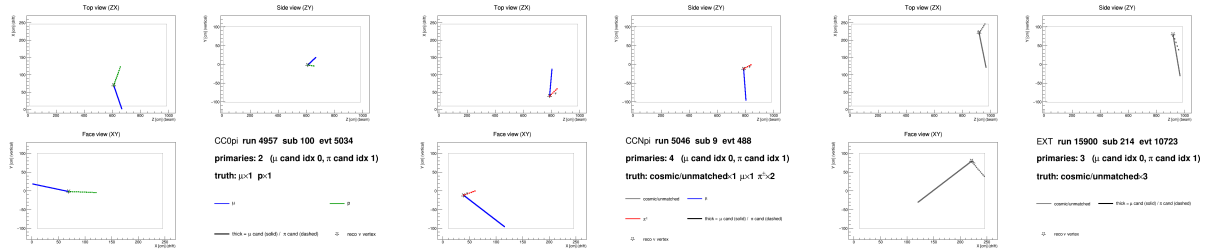
(a) \text{CC}0\pi background: a proton (green, dashed) is reconstructed as the pion candidate. (b) \text{CCN}\pi background: two genuine charged pions present; one is selected as the pion candidate. (c) EXT cosmic event: all tracks are grey (no truth match), faking a neutrino vertex topology.
