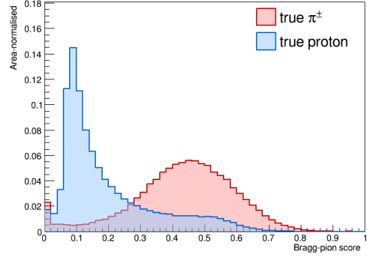
(b) Bragg-pion score (not used).
