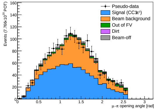
(a) \mu\pi opening angle.
