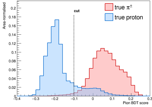
(a) Pion-BDT score; threshold > -0.10 .
