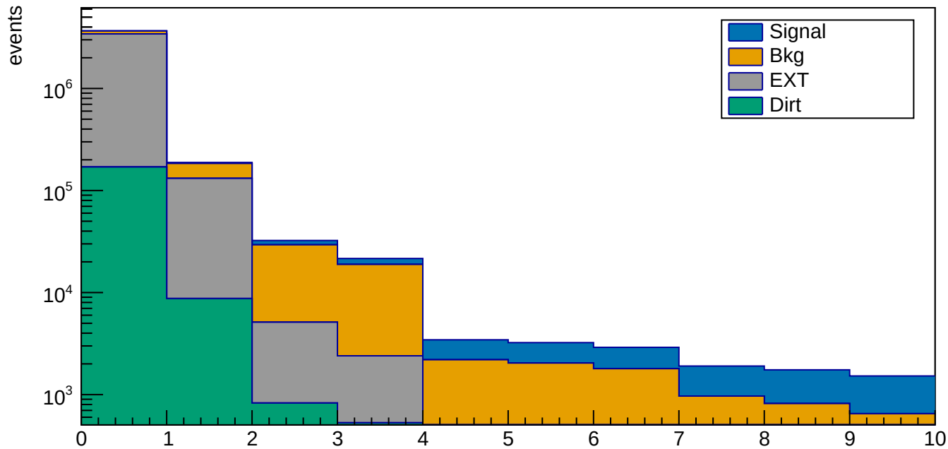
fhc cut-flow
