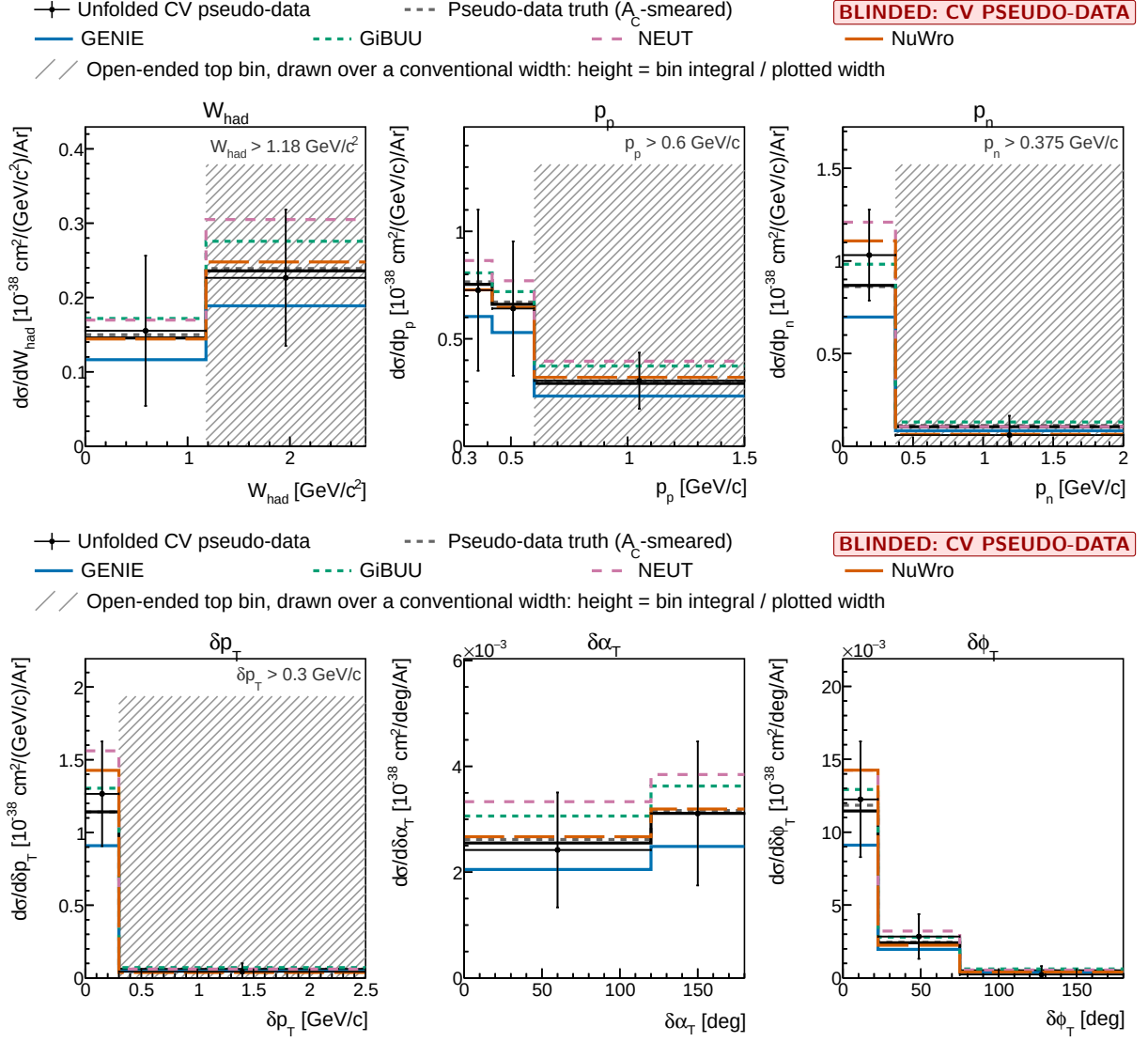
Figure 4: Proton-tagged differential cross sections, FHC: W_{\text{had}} , p_p and p_n (top) and \delta p_T , \delta\alpha_T and \delta\phi_T (bottom). Unfolded pseudo-data (points) are compared with the A_C -smeared pseudo-data truth (grey dashed), the MicroBooNE tune [3] (black) and the GENIE (blue), GiBUU (green), NEUT (purple) and NuWro (orange) predictions for the same phase space. The last bin of each open-ended observable is hatched and labelled with its range; its height is the bin integral divided by the plotted width. \delta\alpha_T rises towards 180^\circ , the signature of final-state interactions.
