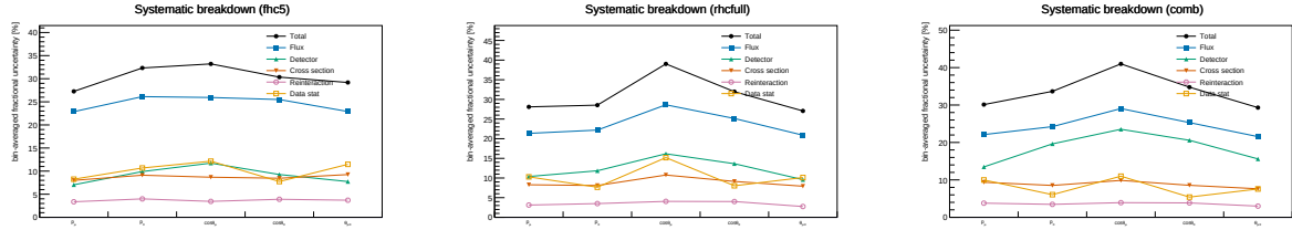
Figure 27: Bin-averaged fractional systematic uncertainty by source vs. observable, for FHC (left), RHC (centre) and combined (right) — the figure form of Tables 28–30. Colours use the Okabe-Ito colourblind-safe palette with distinct markers per source: total (black), flux (blue), detector (green), cross section (vermillion), reinteraction (purple), data stat (orange).
