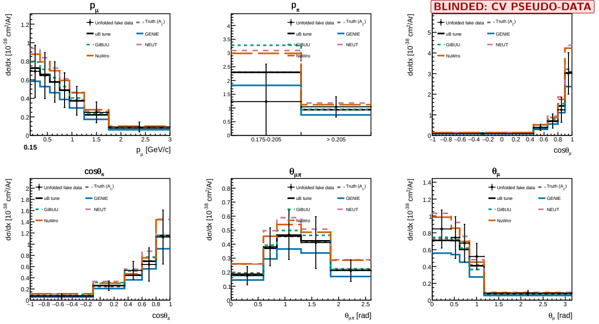
Figure 26: Differential cross sections d\sigma/dx of the six distributions, FHC full exposure, extracted from fake data. The points are the Wiener-SVD estimator A_C x_{\text{true}} ; shown are the unfolded fake data (black points), the A_C -smearred truth of the fake data (grey dashed), the MicroBooNE tune (black solid) and the four generator predictions (GENIE, GiBUU, NEUT, NuWro), all smeared with A_C . The unfolded points recover the injected truth in every observable, the closure summarised in Table 21.
