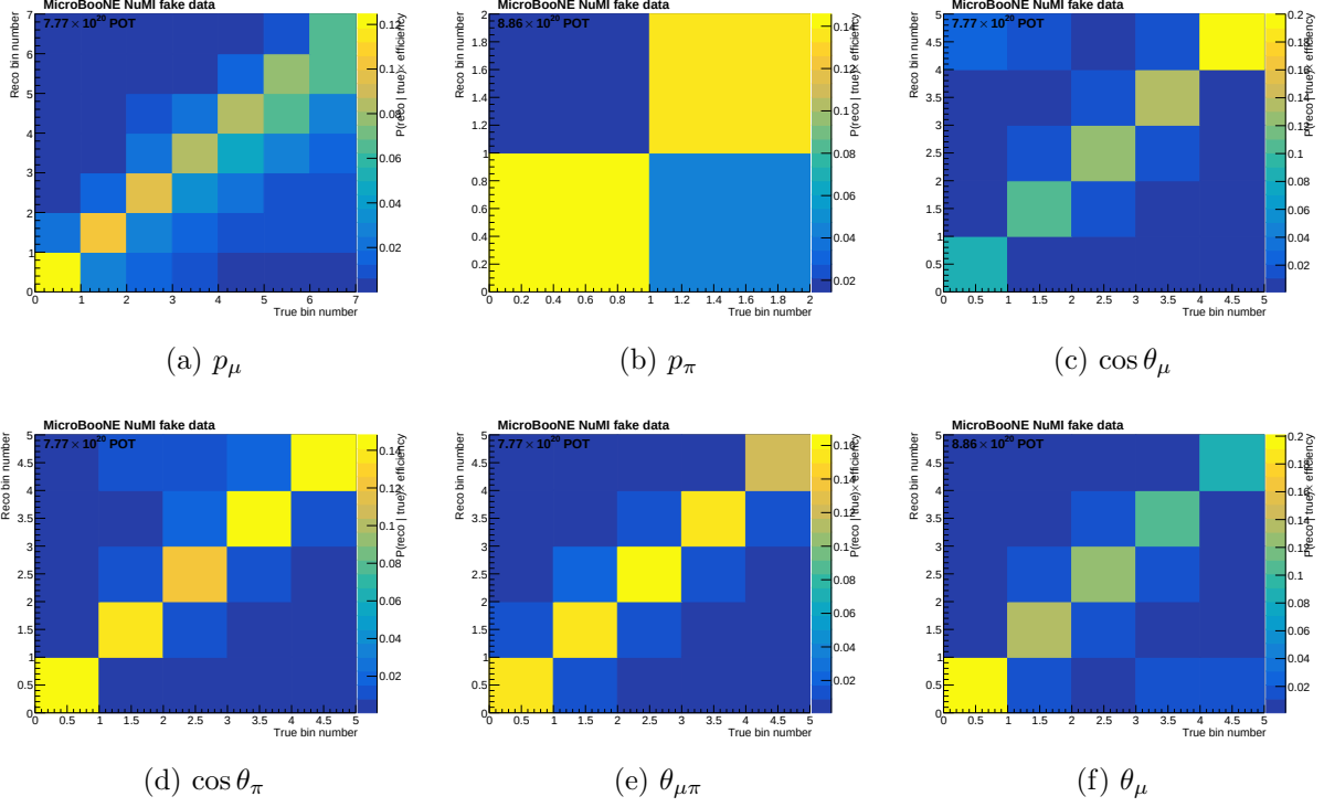
Figure 22: Smearceptance matrices S_{ij} = \varepsilon_j M_{ij} , FHC, exactly as passed to the unfoldr, at the binning of the results, including the two-bin p_\pi response (91% and 76% column-normalised diagonals); the rejected five-bin p_\pi response, which shows the reconstructed events piling into the lowest bin from every true bin, is Fig. 12 of the technical supplement.
