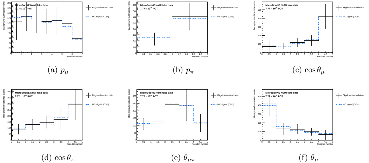
Figure 16: Stage 2, FHC: background-subtracted data compared with the central-value MC signal; the input to the unfolding. RHC: Fig. 18; combined: Fig. 11 of the technical supplement.
