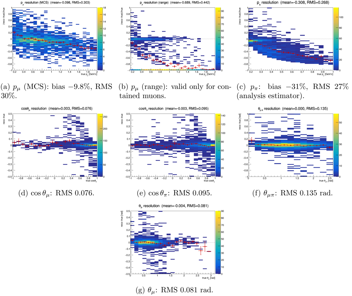
Figure 24: Reconstruction resolution vs. true value, selected signal. Momenta: relative ( \text{reco} - \text{true} )/ \text{true} ; angles: absolute ( \text{reco} - \text{true} ). Red points: mean residual per true bin. \theta_\mu is derived as \arccos(\cos \theta_\mu) , exactly as the bin config does it, so the panel shows the quantity the analysis bins on; it is unbiased ( -0.004 rad) with RMS 0.081 rad, the drift below zero above \sim 2.5 rad being a handful of backward-going muons. The muon MCS momentum slightly over-estimates at low p_\mu and increasingly under-estimates above \sim 1 GeV/c; the range estimator is badly biased for exiting muons (range = distance to wall), which is why the analysis uses range only for contained muons (range-or-MCS). The pion panel shows the estimator the analysis actually bins on, not the raw muon-hypothesis range momentum (Sec. 2.1 of the technical supplement): signed mean bias b = -31\% , RMS 27\% . That average is dominated by high momenta; b is only -2\% in the first true bin and reaches -65\% above 0.8 GeV/c, because the reconstructed value saturates near 0.34 GeV/c once pions interact hadronically before stopping. The angular variables are essentially unbiased with narrow resolution.
