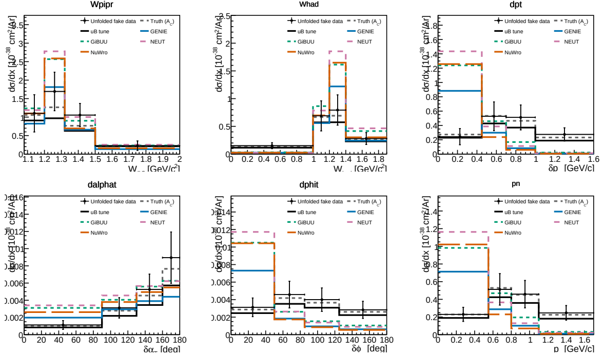
Figure 19: Proton-tagged (CC1 \mu 1 \pi 1 p ) differential cross sections for FHC: the \pi p invariant mass W_{\pi p} , the calorimetric hadronic mass W_{\text{had}} , and the four transverse-kinematic-imbalance observables \delta p_T , \delta \alpha_T , \delta \phi_T and p_n . Unfolded fake data (black points) are compared to the A_C -smeared fake-data truth (grey dashed), the MicroBooNE tune (black), and the GENIE (blue), GiBUU (green), NEUT (purple) and NuWro (orange) predictions built for the same proton-tagged phase space. W_{\pi p} falls from the \Delta(1232) threshold region; \delta \alpha_T rises toward 180^\circ , the signature of final-state interactions.
