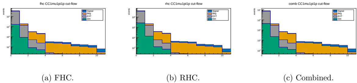
Figure 6: Proton-tagged (CC1mu1pi1p) cut-flow yields at full exposure (log scale; MC-prediction stack, Okabe-Ito: signal blue, background orange, EXT grey, dirt green). The last stage, IdentProton, is the leading-proton identification that defines the proton-tagged sample.
