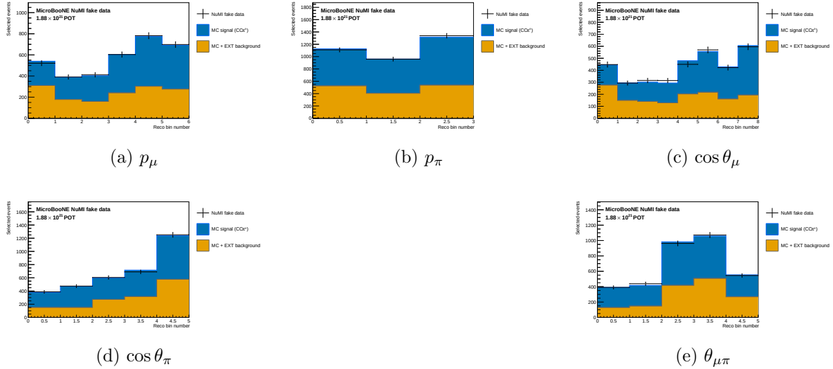
Figure 9: Stage 1, combined: selected reconstructed spectra in the combined configuration.
