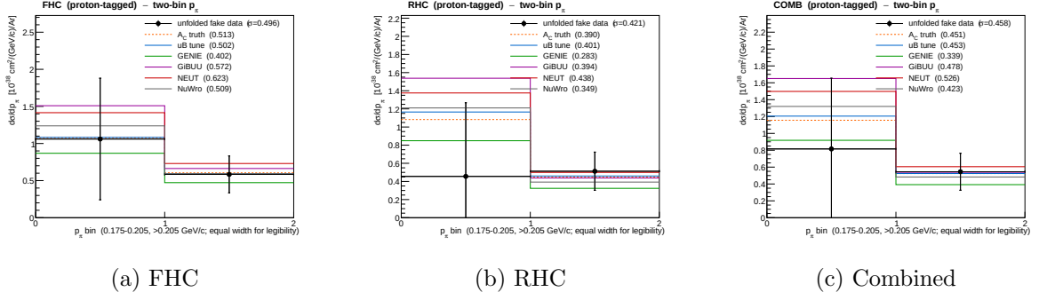
Figure 4: The two-bin p_\pi cross section on the proton-tagged CC1mu1pi1p selection, the graphical form of Tab. 6. The first bin is that of the inclusive result of Fig. 2, and the second is the union of the two upper inclusive regions, since three regions fail the 0.50 criterion in the proton-tagged analysis sample. The bins are drawn equal-width.
