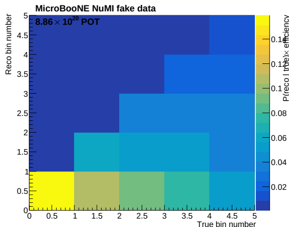
Figure 11: Response matrix of the rejected five-bin p_\pi scheme (FHC, analysis sample): reconstructed events pile into the lowest bin from every true bin (§6.2), which motivated the merged regions of §6.2.5.
