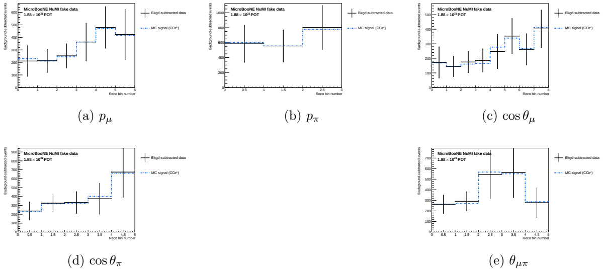
Figure 10: Stage 2, combined: background-subtracted data compared with the central-value MC signal.
