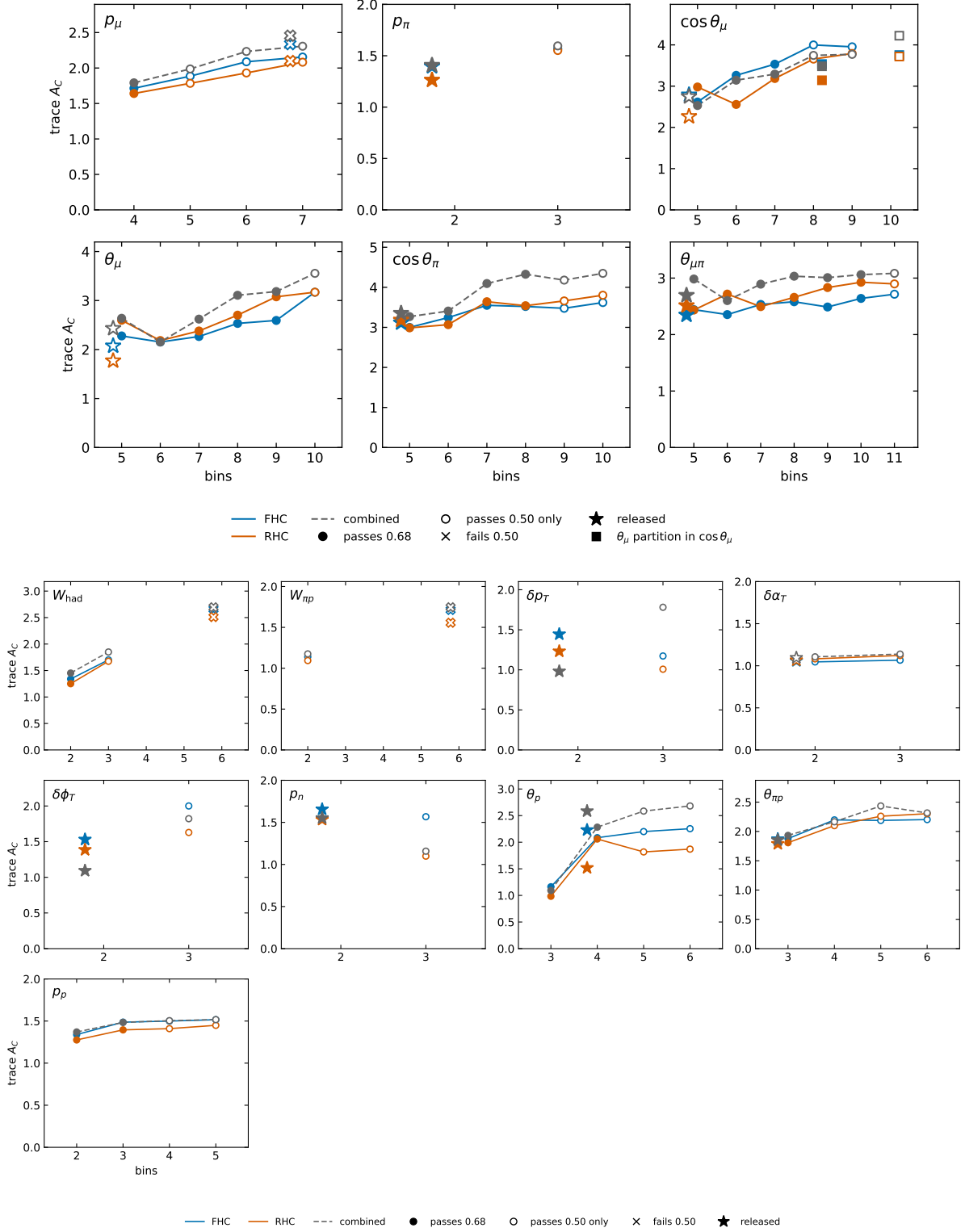
Figure 5: Degrees of freedom for signal (trace of A_C ) against the number of bins, inclusive (top) and proton-tagged (bottom), FHC, RHC and combined. Lines join the maximin binnings; the star is the released binning (for \theta_p and \theta_{np} the study binning), drawn just left of its bin count; squares are the \theta_\mu partitions written in \cos \theta_\mu . A filled marker passes 0.68 in FHC and RHC, an open one 0.50 only, a cross neither. The three-bin W_{\text{had}} is built at an event floor of 30, below that of the family. Pseudo-data; analysis sample.
