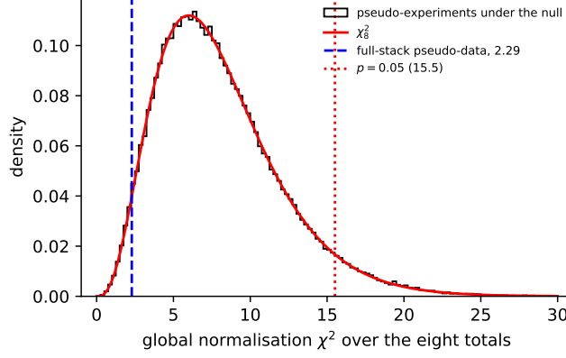
Figure 8: Null calibration of the global normalisation \chi^2 over the eight (region, mode) totals: 2 \times 10^5 pseudo-experiments with the prediction drawn from its pre-fit covariance and Poisson-fluctuated data, against the \chi_8^2 density. The full-stack pseudo-data value, 2.29, is low because those pseudo-data carry none of the prediction’s systematic variation.
