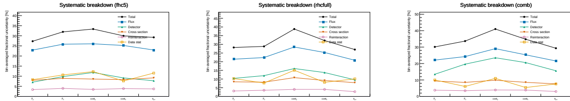
Figure 26: Bin-averaged fractional systematic uncertainty by source vs. observable, for FHC (left), RHC (centre) and combined (right) — the figure form of Tables 24–26. Colours use the Okabe-Ito colourblind-safe palette with distinct markers per source: total (black), flux (blue), detector (green), cross section (vermillion), reinteraction (purple), data stat (orange).
