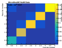
\cos \theta_\mu
