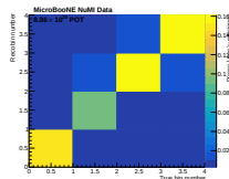
\cos \theta_\pi
