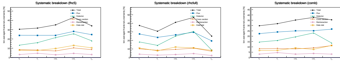
Figure 18: Bin-averaged fractional systematic uncertainty by source vs. observable, for FHC (left), RHC (centre) and combined (right) — the figure form of Tables 16–18. Colours use the Okabe-Ito colourblind-safe palette with distinct markers per source: total (black), flux (blue), detector (green), cross section (vermillion), reinteraction (purple), data stat (orange).
