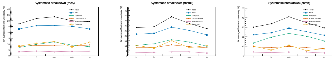
Figure 26: Bin-averaged fractional systematic uncertainty by source vs. observable, for FHC (left), RHC (centre) and combined (right) — the figure form of Tables 25–27. Colours use the Okabe-Ito colourblind-safe palette with distinct markers per source: total (black), flux (blue), detector (green), cross section (vermillion), reinteraction (purple), data stat (orange).
