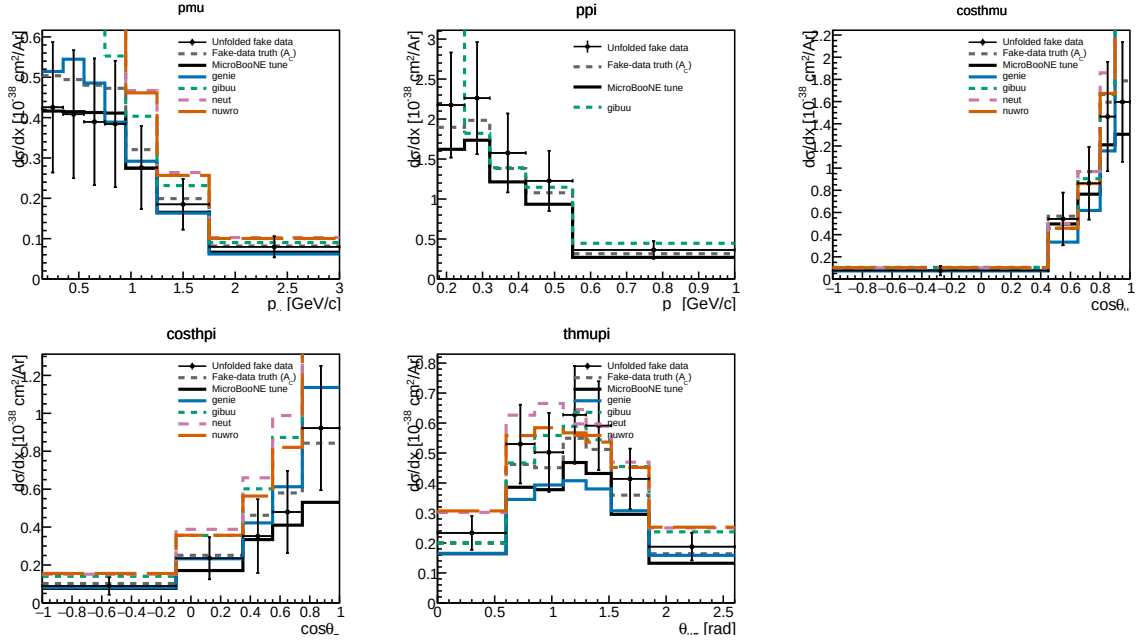
Figure 16: Standalone RHC ( \bar{\nu}_{\mu} -dominant) differential cross sections on the current Poisson-thrown fake data, with the RHC-flux-averaged generator predictions. Same layout as Fig. 15.
