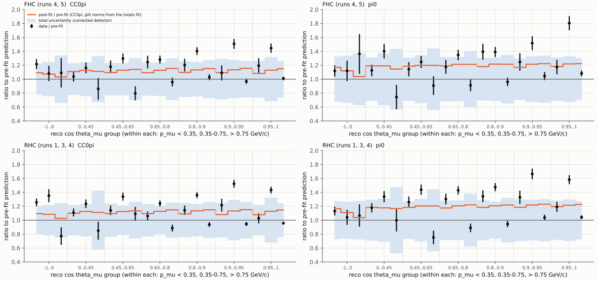
Beam-on control regions (FHC Run 1 excluded): data and post-fit prediction relative to pre-fit
