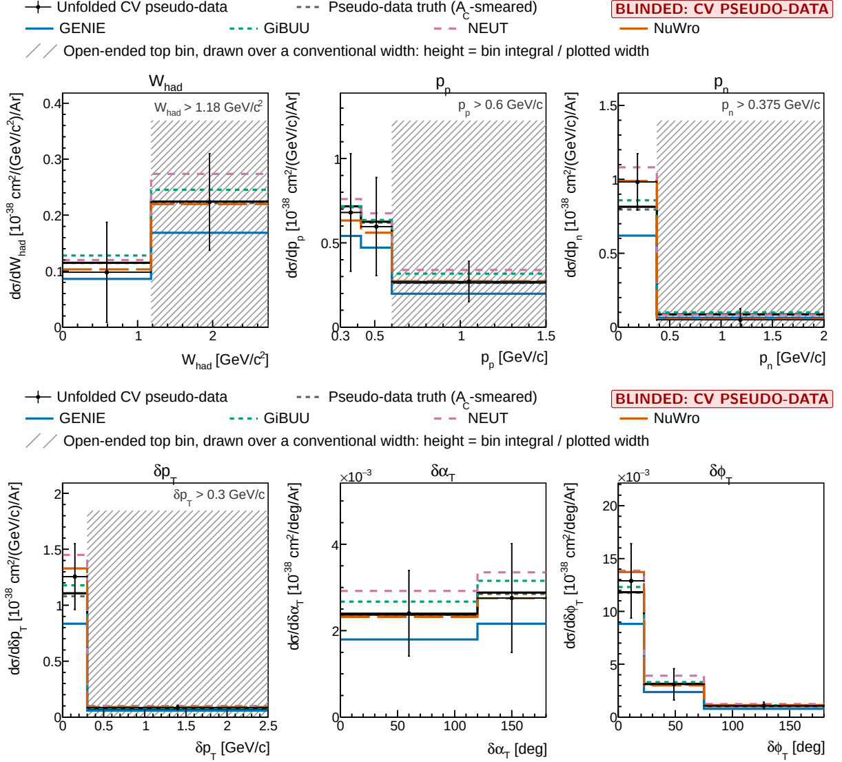
Figure 6: Proton-tagged differential cross sections, the combined configuration: W_{\text{had}} , p_p and p_n (top) and \delta p_T , \delta \alpha_T and \delta \phi_T (bottom). Unfolded pseudo-data (points) are compared with the A_C -smeared pseudo-data truth (grey dashed), the MicroBooNE tune (black) and the GENIE (blue), GiBUU (green), NEUT (purple) and NuWro (orange) predictions for the same phase space. The last bin of each open-ended observable is hatched and labelled with its range; its height is the bin integral divided by the plotted width.
