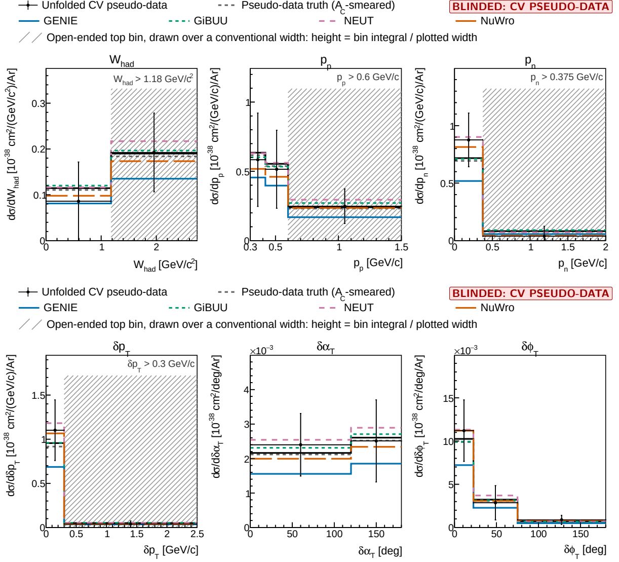
Figure 5: Proton-tagged differential cross sections, RHC: W_{\text{had}} , p_p and p_n (top) and \delta p_T , \delta\alpha_T and \delta\phi_T (bottom). Unfolded pseudo-data (points) are compared with the A_C -smeared pseudo-data truth (grey dashed), the MicroBooNE tune (black) and the GENIE (blue), GiBUU (green), NEUT (purple) and NuWro (orange) predictions for the same phase space. The last bin of each open-ended observable is hatched and labelled with its range; its height is the bin integral divided by the plotted width.
