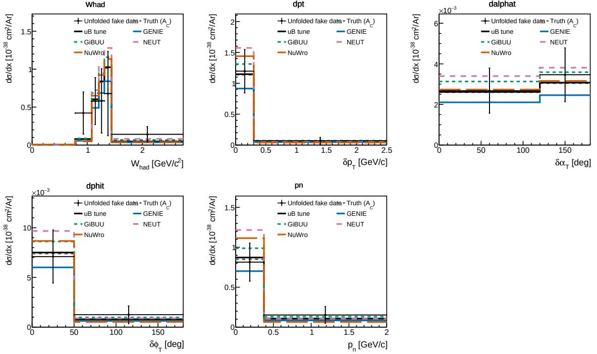
Figure 24: Proton-tagged ( CC1mu1pi1p ) released differential cross sections for FHC: the calorimetric hadronic mass W_{\text{had}} and the four transverse-kinematic-imbalance observables \delta p_T , \delta \alpha_T , \delta \phi_T and p_n (the withdrawn W_{\pi p} shape is not shown; see the technical supplement). Unfolded fake data (black points) are compared to the A_C -smearred fake-data truth (grey dashed), the MicroBooNE tune (black), and the GENIE (blue), GiBUU (green), NEUT (purple) and NuWro (orange) predictions built for the same proton-tagged phase space. \delta \alpha_T rises toward 180^\circ , the signature of final-state interactions.
