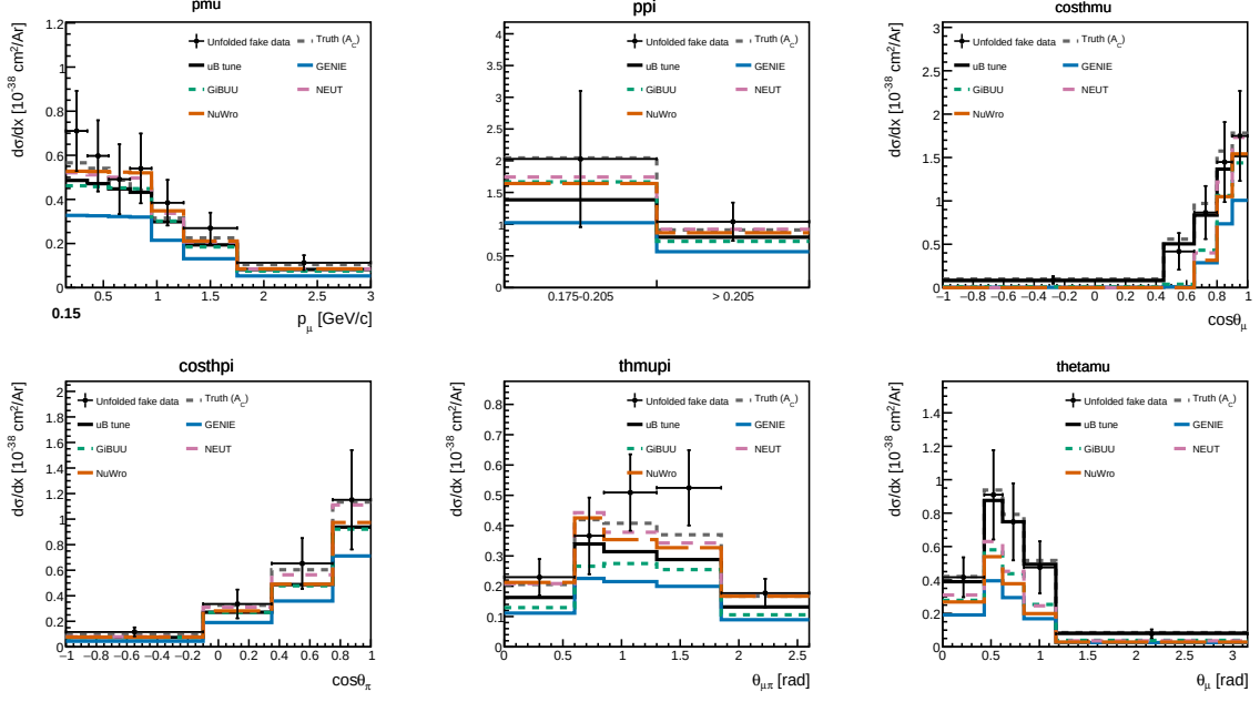
Figure 24: Standalone RHC ( \bar{\nu}_\mu -dominant) differential cross sections on the current Poisson-thrown fake data, with the RHC-flux-averaged generator predictions. Same layout as Fig. 23.
