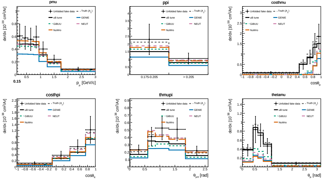
Figure 25: Combined FHC+RHC ( \nu_\mu + \bar{\nu}_\mu ) differential cross sections on the current per-mode-normalised fake data, with the fluence-weighted combined generator predictions.
