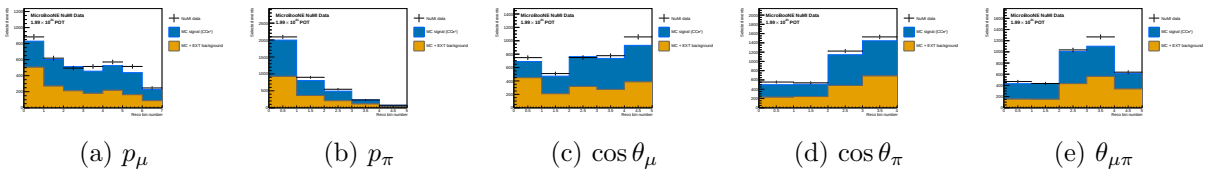
Figure 12: Stage 1, combined: selected reconstructed spectra at the combined FHC+RHC exposure.
