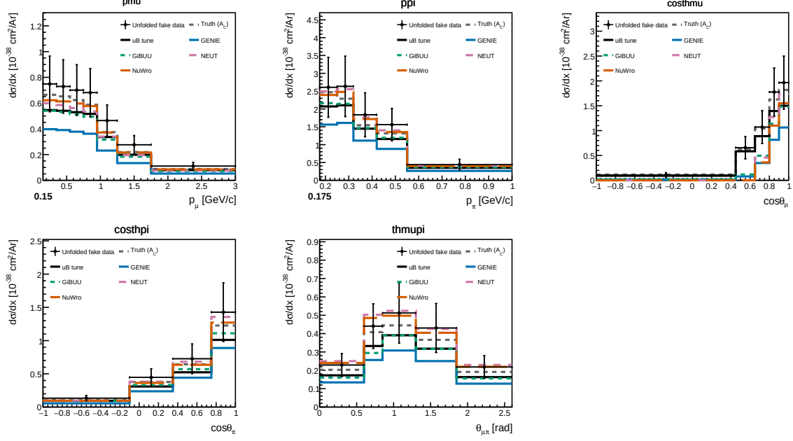
Figure 20: Differential cross sections d\sigma/dx for all five observables on the current Poisson-thrown central-value fake data, FHC full exposure: unfolded fake data (black points), A_C -smearred fake-data truth (grey dashed), the MicroBooNE tune (black solid), and the four generator predictions (GENIE, GiBUU, NEUT, NuWro). The unfolded points recover the injected truth for every observable, the same closure summarised in Tables 19–20.
