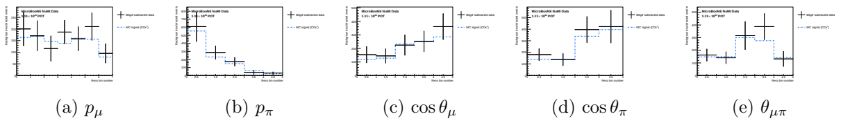
Figure 11: Stage 2, RHC: background-subtracted data compared with the central-value MC signal.
