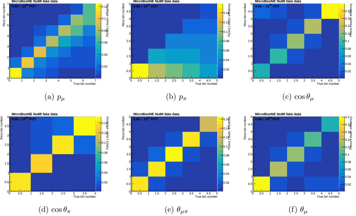
Figure 18: Smearceptance matrices S_{ij} = \varepsilon_j M_{ij} , FHC, exactly as passed to the unfoldr ( plot_step3_smearing_matrix ). Five panels are at the released binning; the p_\pi panel is deliberately the superseded five-bin response, kept as the diagnostic that shows reconstructed events piling into the lowest bin from every true bin and motivated the two-bin scheme (the released two-bin S is 2 \times 2 with column-normalised diagonals 91% and 76%). The colour scale is P(\text{reco} = i | \text{true} = j) \times \varepsilon_j , so each column sums to the selection efficiency of that true bin ( \sim 0.1\text{--}0.2 ), not to unity; the column-normalised migration matrix M is obtained by dividing each column by its sum, and the diagonals quoted in the text are of M . Axes are flat bin numbers (true on x , reco on y ).
