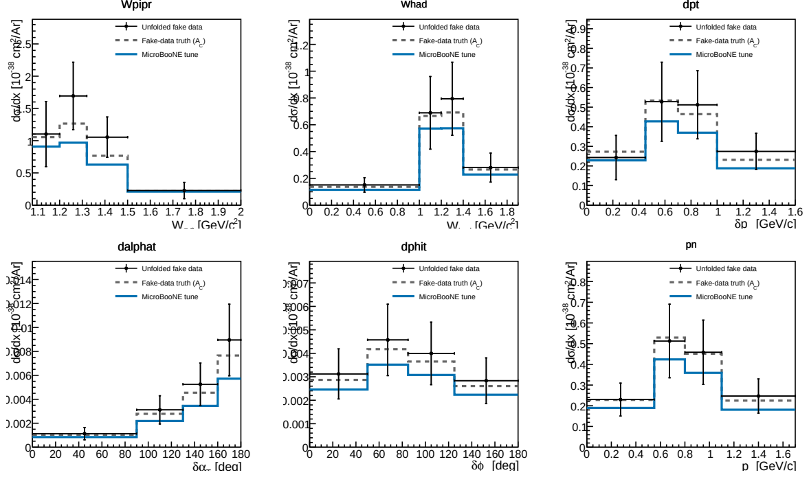
Figure 17: Proton-tagged (CC1mu1pi1p) differential cross sections for FHC: the \pi p invariant mass W_{\pi p} , the calorimetric hadronic mass W_{\text{had}} , and the four transverse-kinematic-imbalance observables \delta p_T , \delta \alpha_T , \delta \phi_T and p_n . Unfolded fake data (black points) are compared to the A_C -smeared fake-data truth (grey dashed) and the MicroBooNE tune (blue). W_{\pi p} falls from the \Delta(1232) threshold region; \delta \alpha_T rises toward 180^\circ , the signature of final-state interactions.
