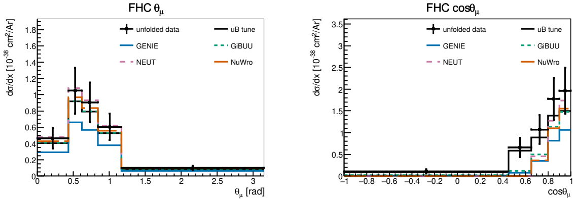
Figure 27: Muon-angle differential cross section in \theta_\mu (left) and \cos \theta_\mu (right), for FHC (top) and RHC (bottom). Unfolded fake data (black points), the MicroBooNE tune (black line) and the four generators are all A_C -smeared. In \cos \theta_\mu the predictions are strongly suppressed by A_C and fall well below both the data and the tune; the most suppressed models are those whose backward bins A_C drives negative. The FHC \theta_\mu panel in this figure predates the regularisation fix: A_C was rank-1 there, so the data and every prediction are the same curve up to normalisation and their apparent agreement carries no shape information. With the width-aware regularisation \theta_\mu discriminates normally (Sec. 9.2).
