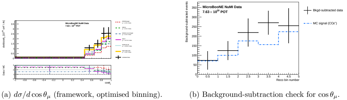
Figure 19: Muon polar angle d\sigma/d\cos\theta_\mu (framework, optimised binning) and the background-subtraction diagnostic. The spectrum rises steeply toward forward angles.
