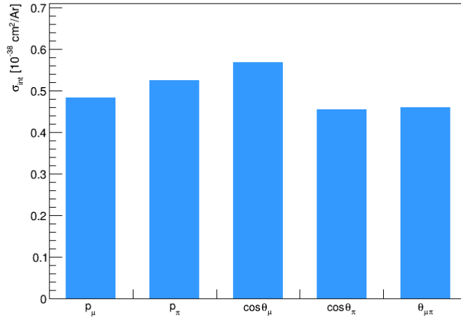
Figure 16: Integrated cross section \sigma_{\text{int}} from each of the five observables (framework Wiener-SVD, optimised binning, GENIE detVar-CV fake data). Total uncertainty (full covariance); optimised binning. The values differ between observables because each integrates a different projection of the same restricted phase space.
