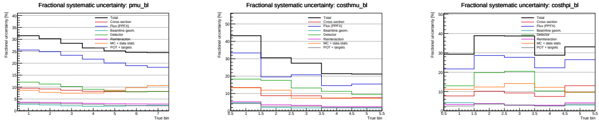
Figure 15: Fractional systematic uncertainty by source (optimised binning): total (black), cross section (red), flux/beamline (blue), detector (green), reinteraction (magenta), MC+data stats (orange), POT+targets (grey).
