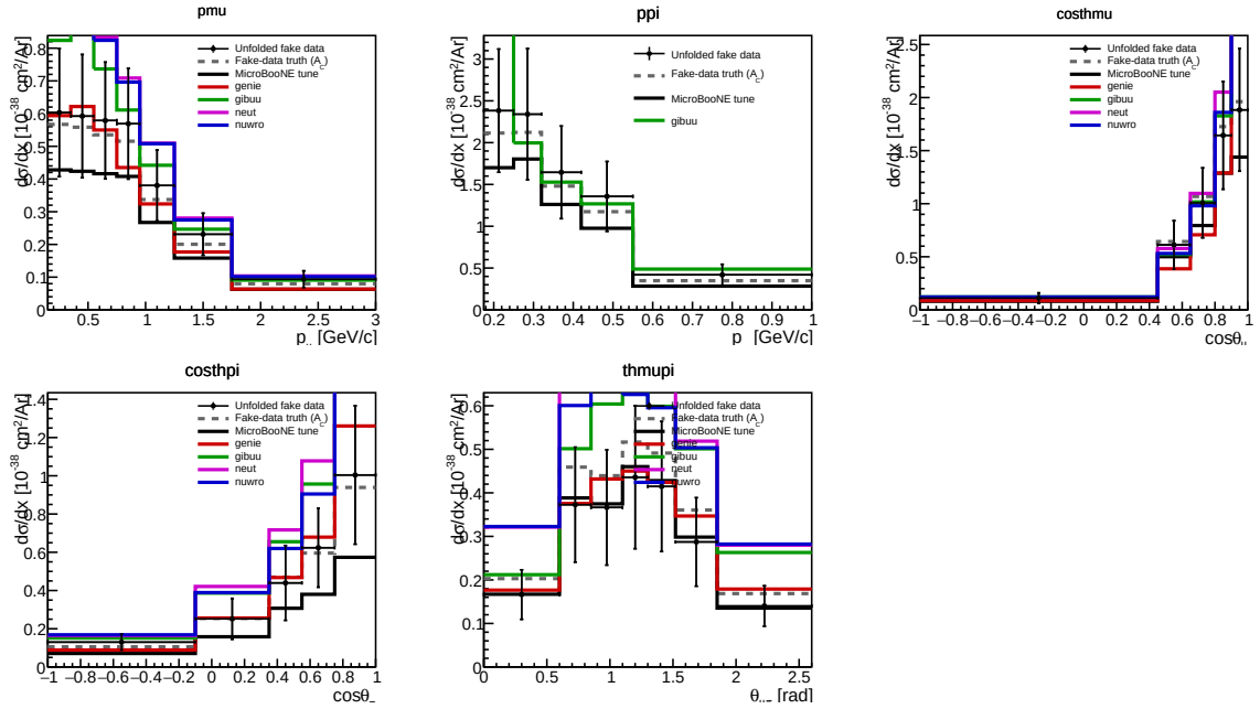
Figure 14: Combined FHC+RHC ( \nu_{\mu} + \bar{\nu}_{\mu} ) differential cross sections on the current per-mode-normalised fake data, with the fluence-weighted combined generator predictions. The standalone RHC result ( dsigma_RHCFULL ) is obtained identically.
