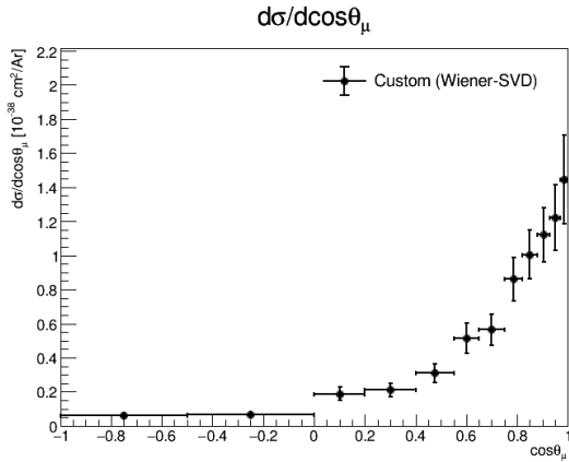
(a) d\sigma/d\cos\theta_\mu (custom, measured phase space).
