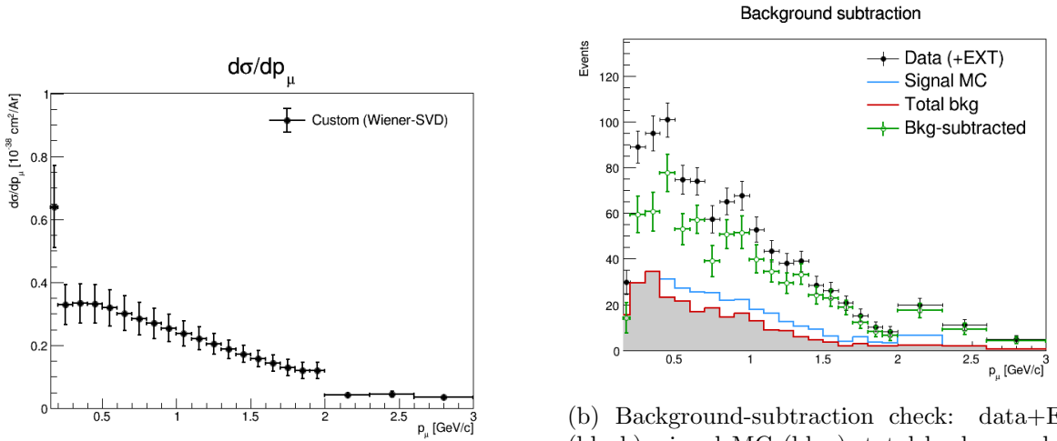
(a) d\sigma/dp_\mu (custom, measured phase space).
