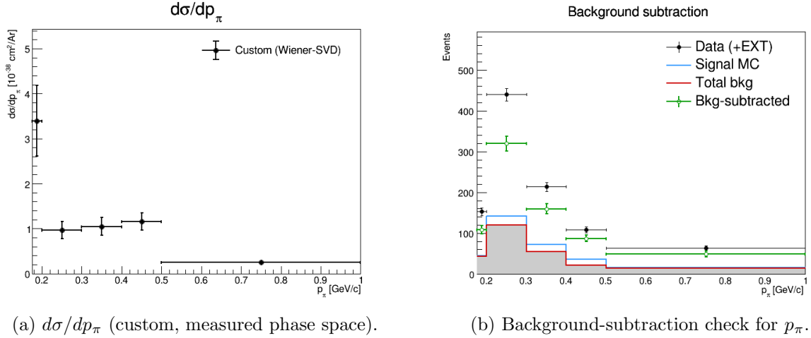
Figure 15: Pion momentum d\sigma/dp_\pi unfolding diagnostics.
