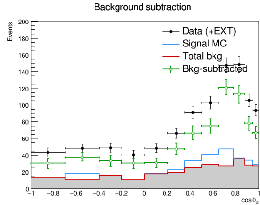
(b) Background-subtraction check for \cos\theta_\pi .
