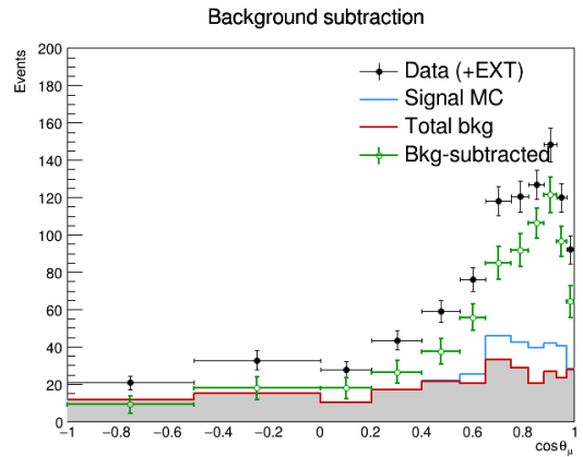
(b) Background-subtraction check for \cos\theta_\mu .
