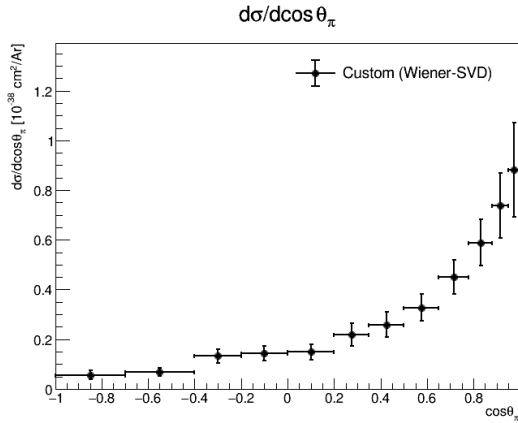
(a) d\sigma/d\cos\theta_\pi (custom, measured phase space).
