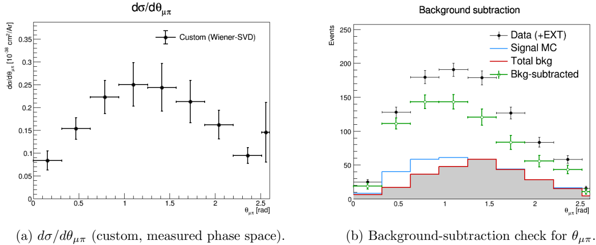
Figure 18: Opening angle d\sigma/d\theta_{\mu\pi} unfolding diagnostics.
