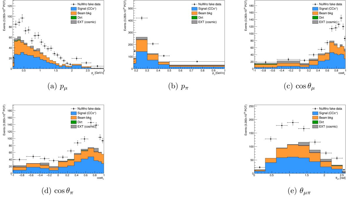
Figure 9: Reconstructed-space spectra at the final cut for all five observables. NuWro fake data (black points), stacked signal (blue), beam background (orange), dirt (green), and EXT (grey). NuWro carries roughly twice the GENIE-predicted signal, consistent with the generator spread in \text{CC}\pi^+ production.
