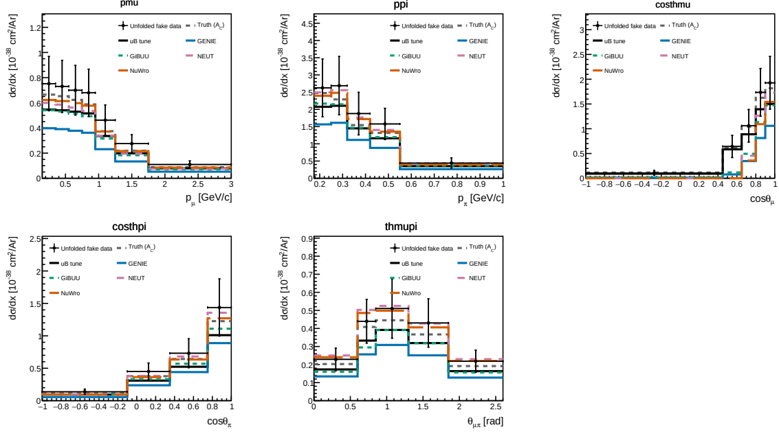
Figure 14: Differential cross sections d\sigma/dx for all five observables on the current Poisson-thrown central-value fake data, FHC full exposure: unfolded fake data (black points), A_C -smearred fake-data truth (grey dashed), the MicroBooNE tune (black solid), and the four generator predictions (GENIE, GiBUU, NEUT, NuWro). The unfolded points recover the injected truth for every observable, the same closure summarised in Tables 16–17.
