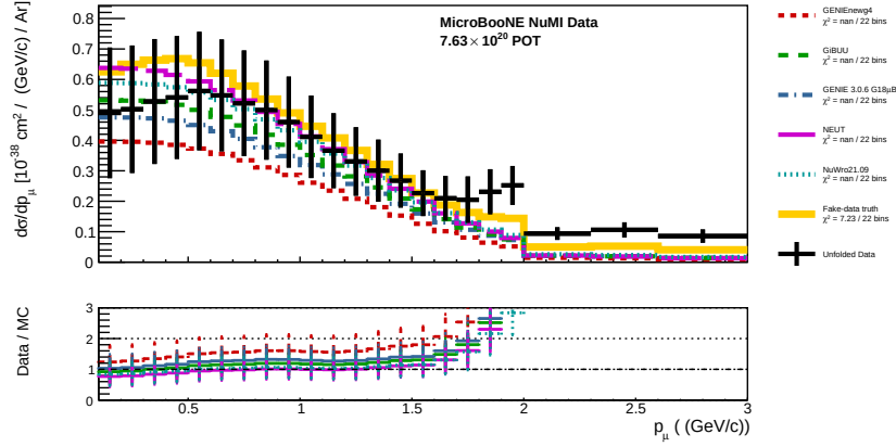
Figure 37: Unfolded d\sigma/dp_\mu (fake data): four generators + MicroBooNE tune + fake-data truth (all A_C -smeared), with data/MC ratio panel.
