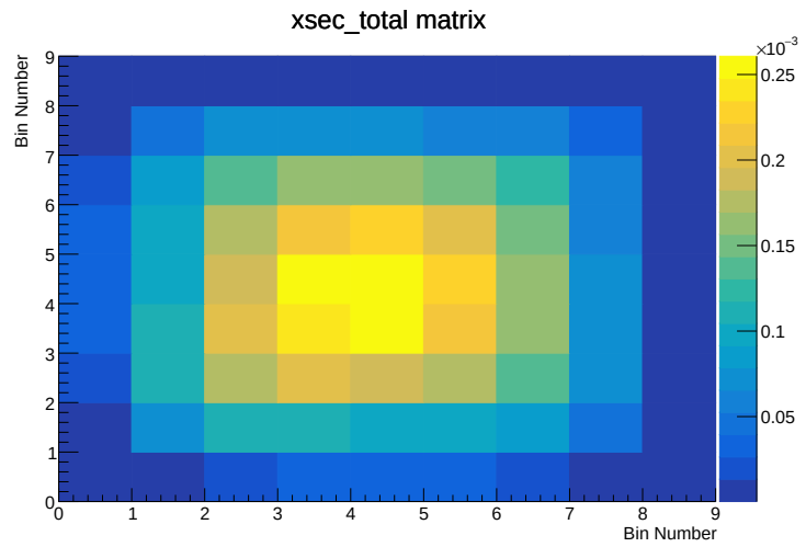
Figure 27: GENIE cross-section (UBGenie + unisim) covariance.
