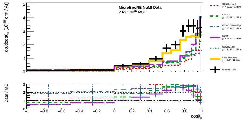
Figure 39: Unfolded d\sigma/d\cos\theta_\mu .
