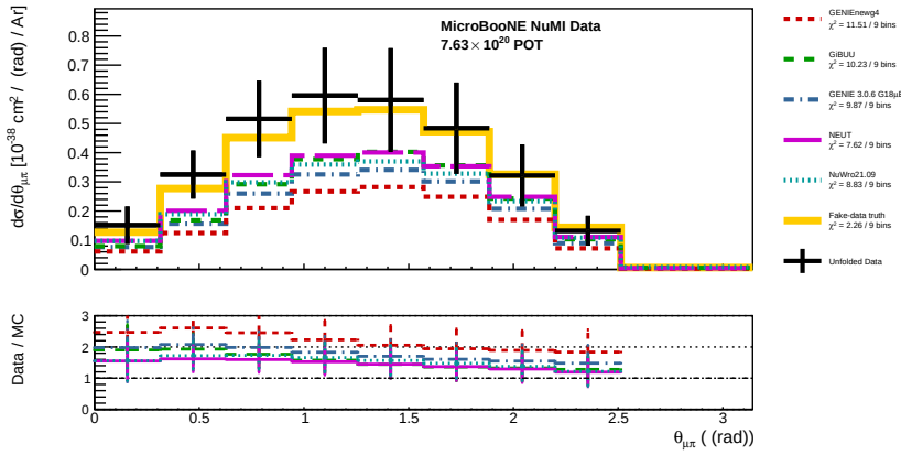
Figure 41: Unfolded d\sigma/d\theta_{\mu\pi} .
