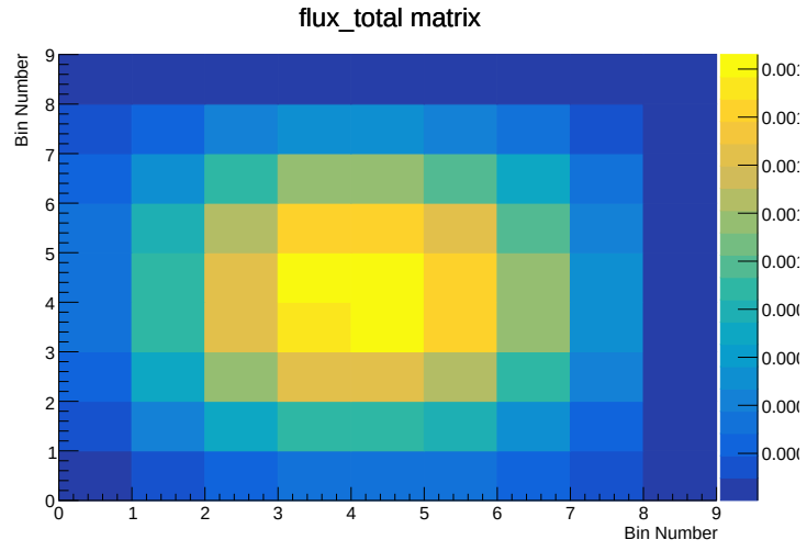
Figure 26: Flux (PPFX) covariance.
