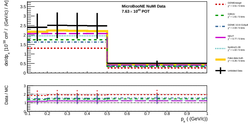
Figure 38: Unfolded d\sigma/dp_\pi .
