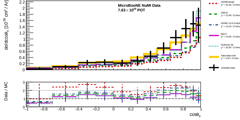
Figure 40: Unfolded d\sigma/d\cos\theta_\pi .
