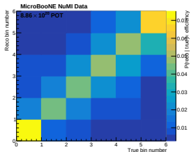
\delta \alpha_T
