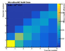
\delta p_T
