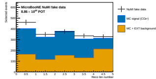
\theta_\mu
