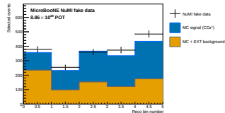
\cos \theta_\mu
