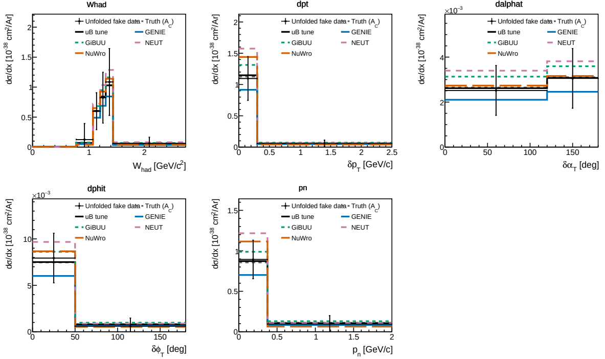
Figure 29: Proton-tagged ( CC1mu1pi1p ) released differential cross sections for FHC: the calorimetric hadronic mass W_{\text{had}} and the four transverse-kinematic-imbalance observables \delta p_T , \delta\alpha_T , \delta\phi_T and p_n (the withdrawn W_{\pi p} shape is not shown; see the technical supplement). Unfolded fake data (black points) are compared to the A_C -smearred fake-data truth (grey dashed), the MicroBooNE tune (black), and the GENIE (blue), GiBUU (green), NEUT (purple) and NuWro (orange) predictions built for the same proton-tagged phase space. \delta\alpha_T rises toward 180^\circ , the signature of final-state interactions.
