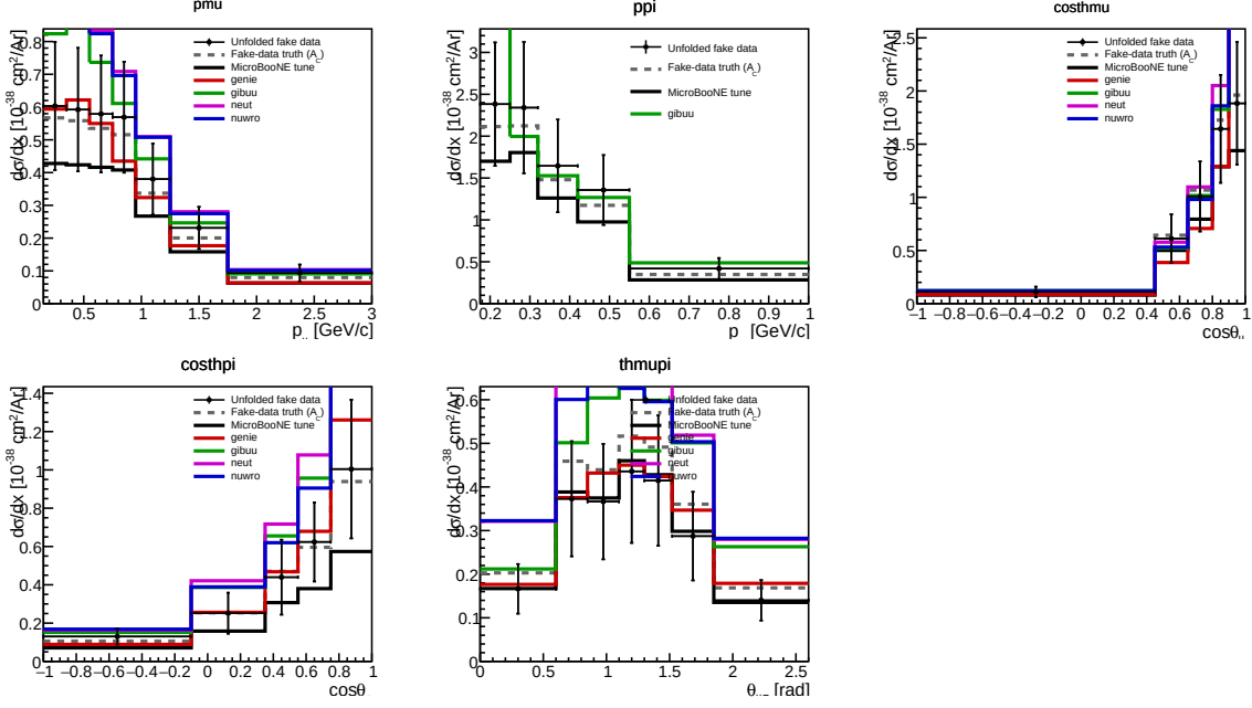
Figure 22: Combined FHC+RHC ( \nu_\mu + \bar{\nu}_\mu ) differential cross sections on the current per-mode-normalised fake data, with the fluence-weighted combined generator predictions. The standalone RHC result (dsigma_RHCFULL) is obtained identically.
