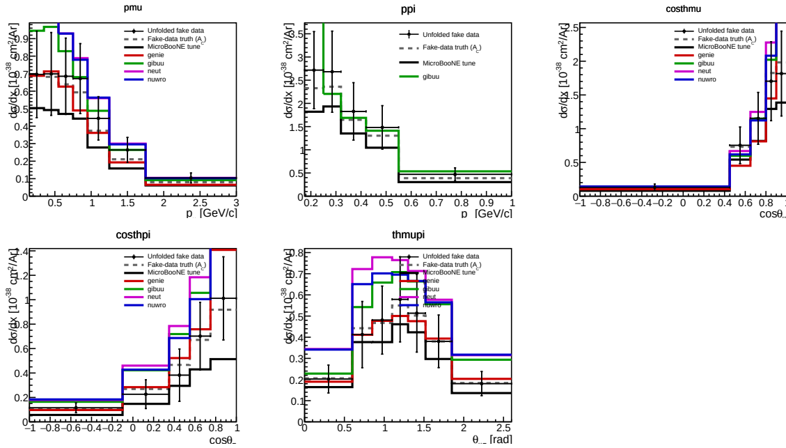
Figure 21: Differential cross sections d\sigma/dx for all five observables on the current Poisson-thrown central-value fake data, FHC full exposure: unfolded fake data (black points), A_C -smeared fake-data truth (grey dashed), the MicroBooNE tune (black solid), and the four generator predictions (GENIE, GiBUU, NEUT, NuWro). The unfolded points recover the injected truth for every observable, the same closure summarised in Tables 27–28.
