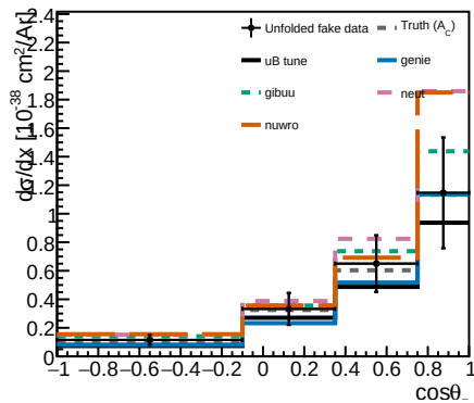
costhpi
