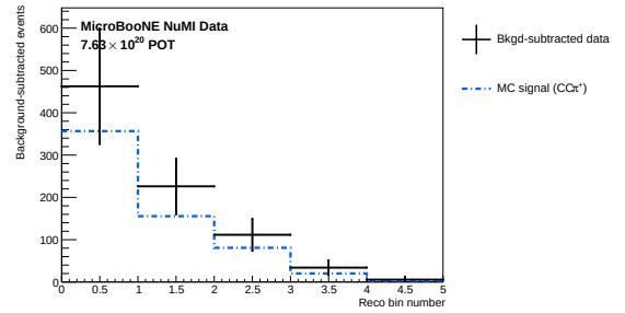
(b) Background-subtraction check for p_\pi .
