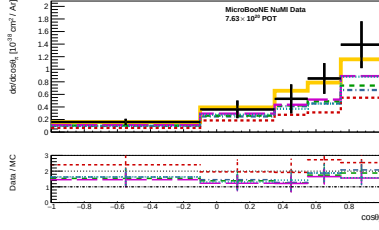
(a) d\sigma/d\cos\theta_\pi (framework, optimised binning).
