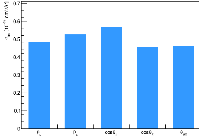
Figure 19: Integrated cross section \sigma_{\text{int}} from each of the five observables (framework Wiener-SVD, optimised binning, GENIE detVar-CV fake data). Total uncertainty (full covariance); optimised binning. The values differ between observables because each integrates a different projection of the same restricted phase space.
