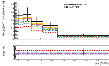
(a) d\sigma/dp_\pi (framework, optimised binning).
