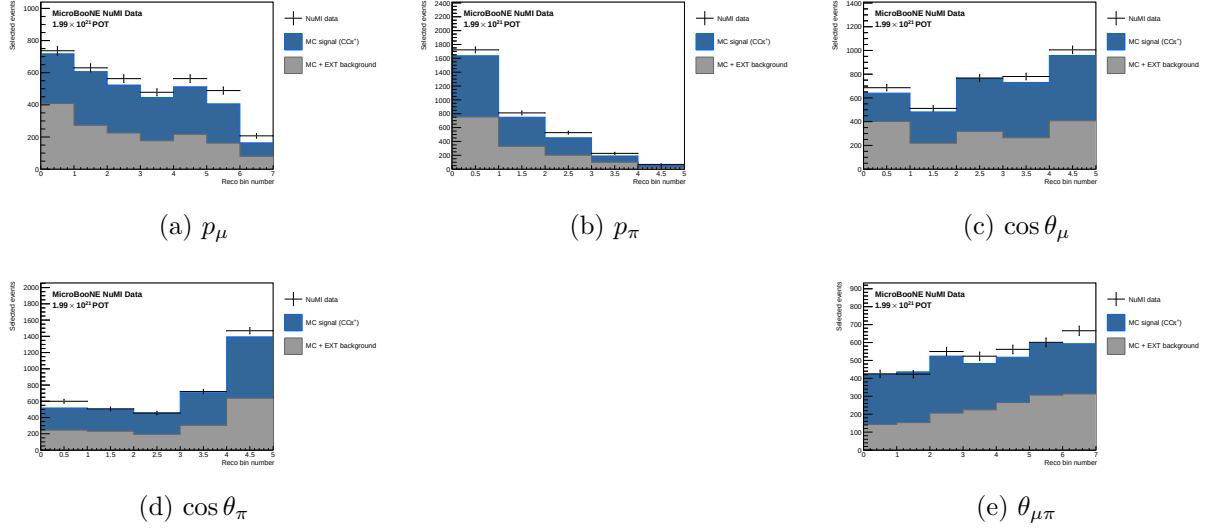
Figure 11: Reconstructed-space spectra, combined FHC+RHC (per-mode normalised); same components as Fig. 9.
