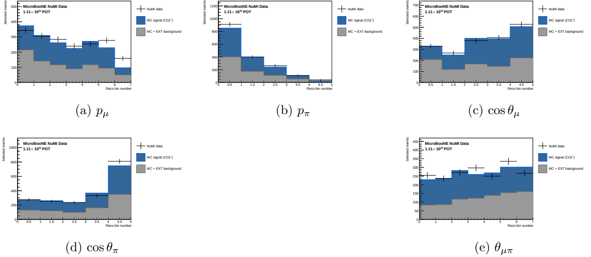
Figure 10: Reconstructed-space spectra, RHC full exposure (Runs 1+2+3+4a+4b+4c); same components as Fig. 9.
