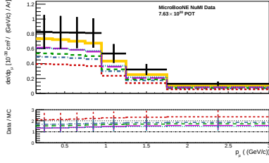
(a) d\sigma/dp_\mu (framework, optimised binning).
