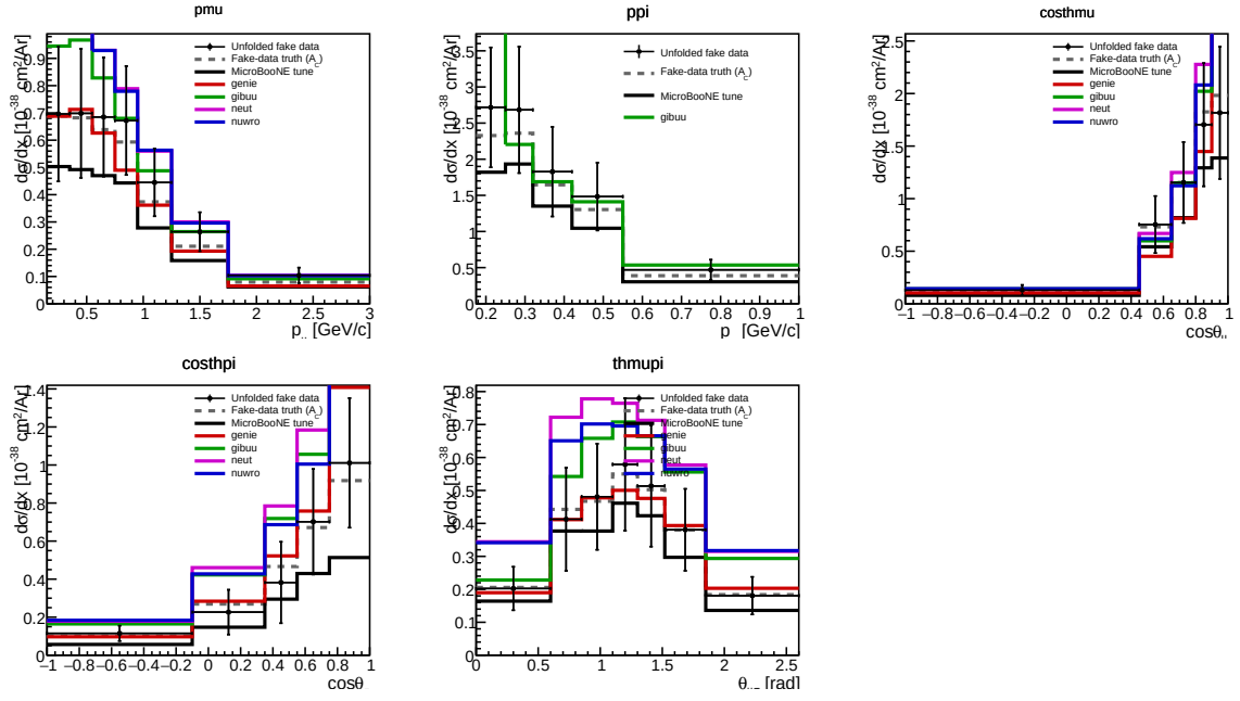
Figure 15: Differential cross sections d\sigma/dx for all five observables on the current Poisson-thrown central-value fake data, FHC full exposure: unfolded fake data (black points), A_C -smeared fake-data truth (grey dashed), the MicroBooNE tune (black solid), and the four generator predictions (GENIE, GiBUU, NEUT, NuWro). The unfolded points recover the injected truth for every observable, the same closure summarised in Tables 12–13.
