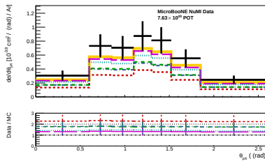
(a) d\sigma/d\theta_{\mu\pi} (framework, optimised binning).
