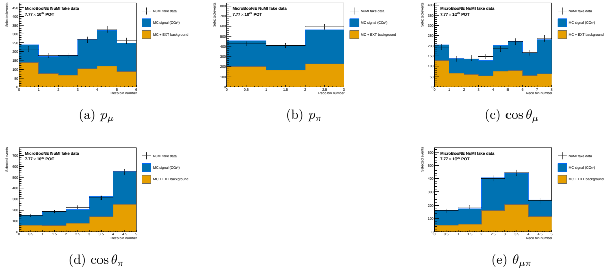
Figure 12: Stage 1, FHC: selected reconstructed spectra scaled to the full exposure, with the MC split into signal and background. Points are the Poisson-thrown fake data. The RHC equivalent is Fig. 14 and the combined one Fig. 14 of the technical supplement.
