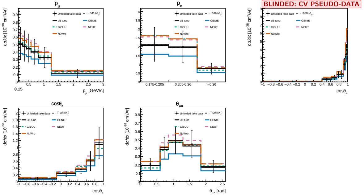
Figure 24: RHC differential cross sections from fake data, with the generator predictions averaged over the RHC flux. Same layout as Fig. 23.
