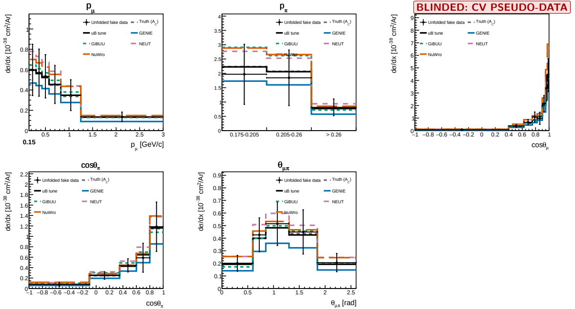
Figure 25: Combined FHC+RHC differential cross sections from fake data normalised per horn mode, with the fluence-weighted combination of the generator predictions. Same layout as Fig. 23.
