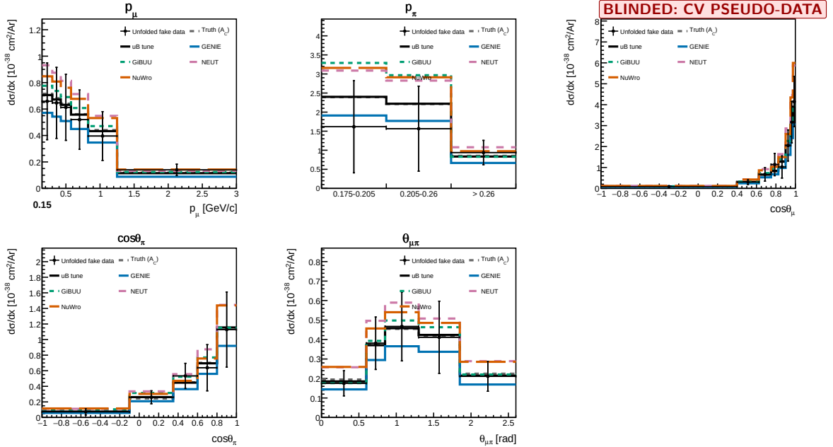
Figure 23: Differential cross sections d\sigma/dx of the five distributions, FHC full exposure, extracted from fake data. The points are the Wiener-SVD estimator A_C x_{\text{true}} ; shown are the unfolded fake data (black points), the A_C -smeared truth of the fake data (grey dashed), the MicroBooNE tune (black solid) and the four generator predictions (GENIE, GiBUU, NEUT, NuWro), all smeared with A_C . The unfolded points recover the injected truth in every observable, the closure summarised in Table 20.
