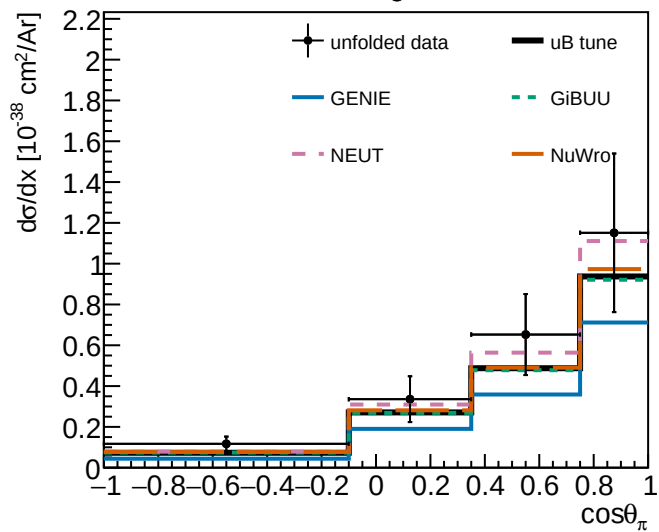
RHC costhpi ( A_C -smeared)
