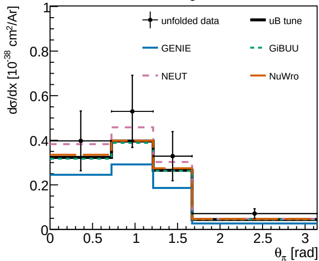
RHC thetapi ( A_C -smeared)
