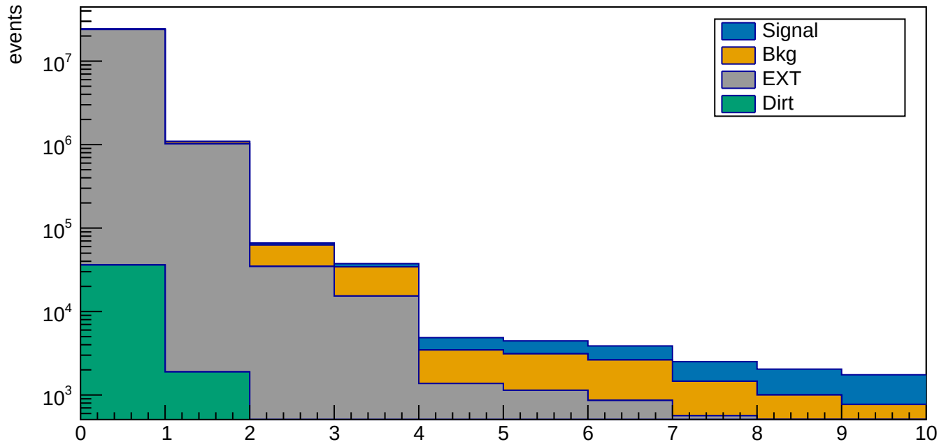
fhc cut-flow
