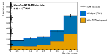
\cos \theta_\pi
