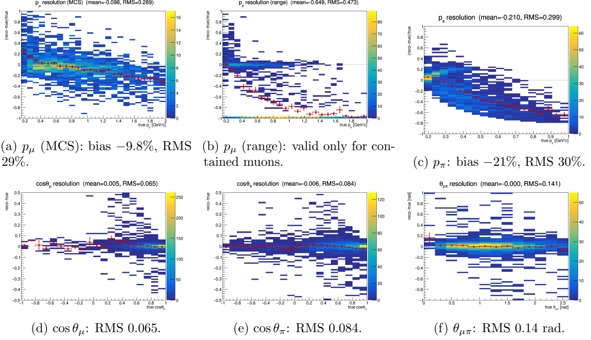
Figure 12: Reconstruction resolution vs. true value, selected signal. Momenta: relative ( \text{reco} - \text{true} )/true; angles: absolute ( \text{reco} - \text{true} ). Red points: mean residual per true bin. The muon MCS momentum slightly over-estimates at low p_\mu and increasingly under-estimates above \sim 1 GeV/c; the range estimator is badly biased for exiting muons (range = distance to wall), which is why the analysis uses range only for contained muons (range-or-MCS). The pion momentum (proton-hypothesis range KE) under-estimates true p_\pi by \sim 21\% . The angular variables are essentially unbiased with narrow resolution.
