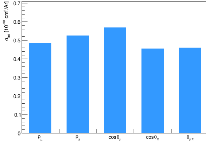
Figure 13: Integrated cross section \sigma_{\text{int}} from each of the five observables (custom Wiener-SVD, measured phase space, NuWro fake data). Total uncertainty (full covariance); optimised binning. The values differ between observables because each integrates a different projection of the same restricted phase space.
