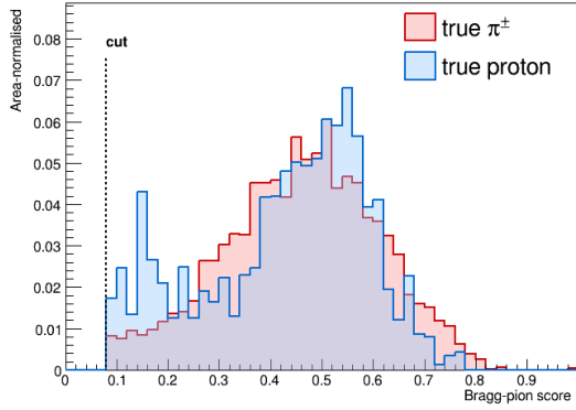
(a) Bragg-pion score ( trk_bragg_pion_v ). Working-point threshold: \geq 0.08 .
