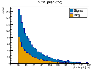
(c) Pion length, FHC.
