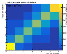
\delta\alpha_T
