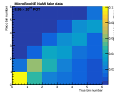
\delta\rho_T
