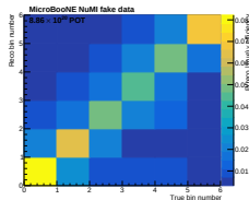
\delta\phi_T
