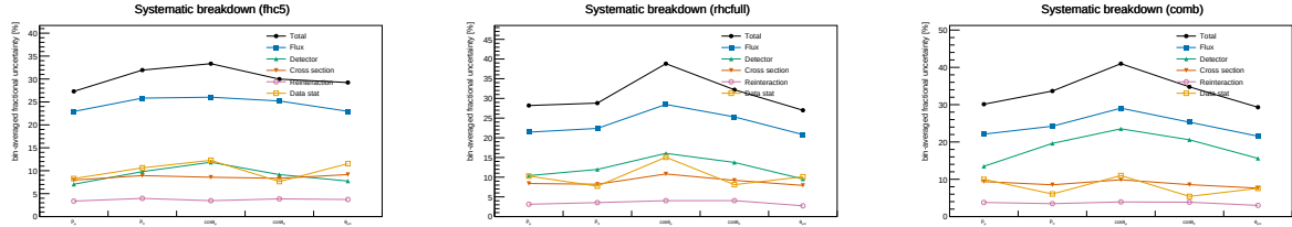
Figure 20: Bin-averaged fractional systematic uncertainty by source vs. observable, for FHC (left), RHC (centre) and combined (right) — the figure form of Tables 21–23. Colours use the Okabe-Ito colourblind-safe palette with distinct markers per source: total (black), flux (blue), detector (green), cross section (vermillion), reinteraction (purple), data stat (orange).
