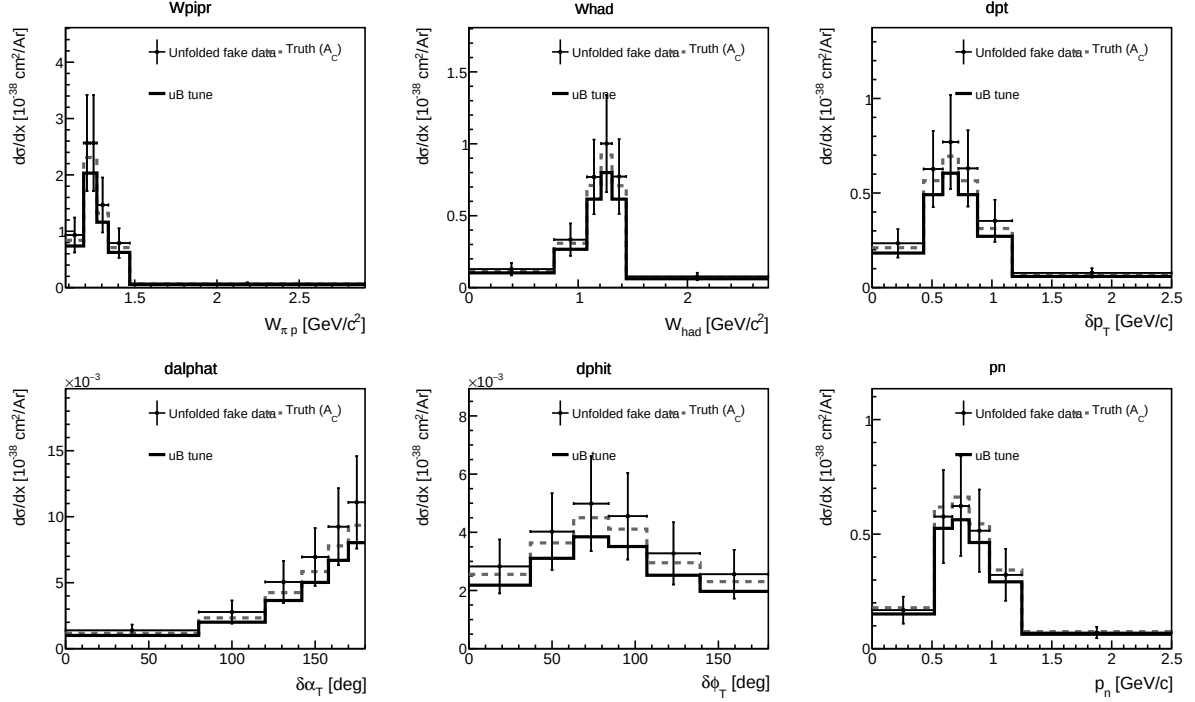
Figure 19: Proton-tagged (CC1mu1pi1p) differential cross sections for FHC: the \pi p invariant mass W_{\pi p} , the calorimetric hadronic mass W_{\text{had}} , and the four transverse-kinematic-imbalance observables \delta p_T , \delta \alpha_T , \delta \phi_T and p_n . Unfolded fake data (black points) are compared to the A_C -smeared fake-data truth (grey dashed), the MicroBooNE tune (black), and the GENIE (blue), GiBUU (green), NEUT (purple) and NuWro (orange) predictions built for the same proton-tagged phase space. W_{\pi p} falls from the \Delta(1232) threshold region; \delta \alpha_T rises toward 180^\circ , the signature of final-state interactions.
