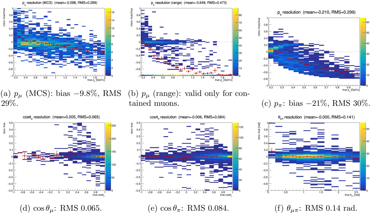
Figure 13: Reconstruction resolution vs. true value, selected signal. Momenta: relative ( \text{reco} - \text{true} )/true; angles: absolute ( \text{reco} - \text{true} ). Red points: mean residual per true bin. The muon MCS momentum slightly over-estimates at low p_\mu and increasingly under-estimates above \sim 1 GeV/ c ; the range estimator is badly biased for exiting muons (range = distance to wall), which is why the analysis uses range only for contained muons (range-or-MCS). The pion momentum (proton-hypothesis range KE) under-estimates true p_\pi by \sim 21\% . The angular variables are essentially unbiased with narrow resolution.
