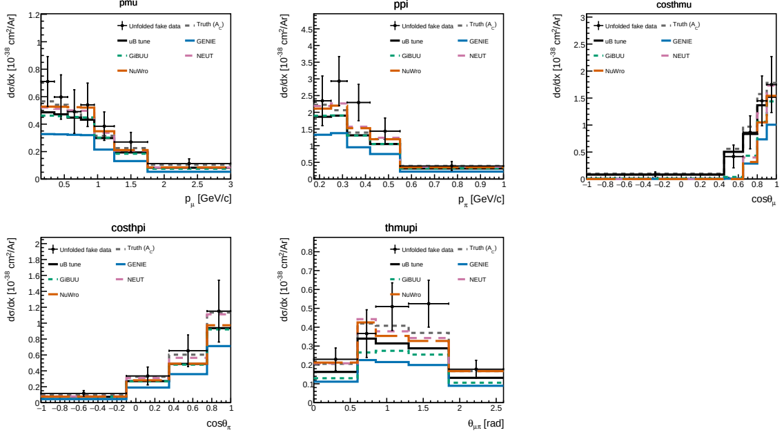
Figure 15: Standalone RHC ( \bar{\nu}_\mu -dominant) differential cross sections on the current Poisson-thrown fake data, with the RHC-flux-averaged generator predictions. Same layout as Fig. 14.
