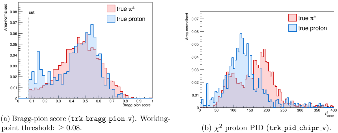
Figure 5: Pion-candidate PID distributions for true \pi^\pm (red) and true protons (blue) at the final cut stage. The Bragg-pion score provides the primary proton rejection; \chi^2_p is studied as cross-check.
