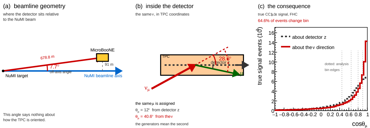
Figure 1: The NuMI geometry seen by MicroBooNE. (a) Beamline geometry, to scale: the detector sits 91.1 m off the NuMI axis at a baseline of 678.8 m, an off-axis angle of 7.7^\circ . (b) The same neutrinos in TPC coordinates, to scale (the x – z projection; the quoted 28.6^\circ is the full three-dimensional angle): the beam arrives 28.6^\circ away from the detector z axis, so one and the same muon is assigned \theta_\mu = 12^\circ about z but \theta_\mu = 40.6^\circ about the neutrino. The generators mean the second. (c) The resulting shift in the true \cos \theta_\mu distribution; dotted lines mark the analysis bin edges. Under the two conventions 64.6% of signal events fall in a different bin (44.6% for \cos \theta_\pi ).
