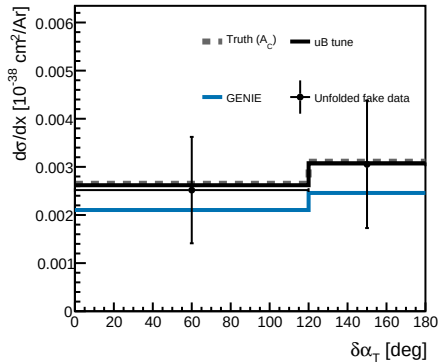
dalphot
