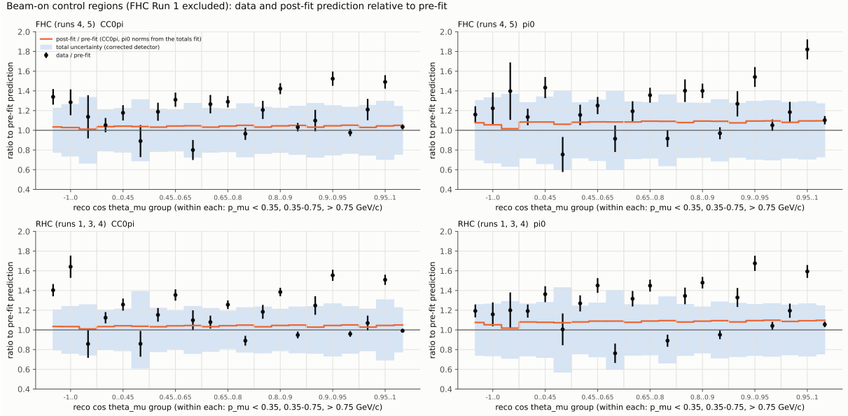
Figure 5: Beam-on control regions without FHC Run 1: data and the post-fit prediction (CC0 \pi and \pi^0 normalisations from the totals fit) relative to the pre-fit prediction, in reconstructed \cos \theta_\mu groups, each split into p_\mu < 0.35 , 0.35\text{--}0.75 and > 0.75 GeV/c; band: total uncertainty.
