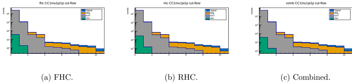
Figure 17: Proton-tagged ( CC1\mu1\pi1p ) cut-flow yields at full exposure (log scale; MC-prediction stack, Okabe-Ito: signal blue, background orange, EXT grey, dirt green). The last stage, IdentProton, is the leading-proton identification that defines the subsample.
