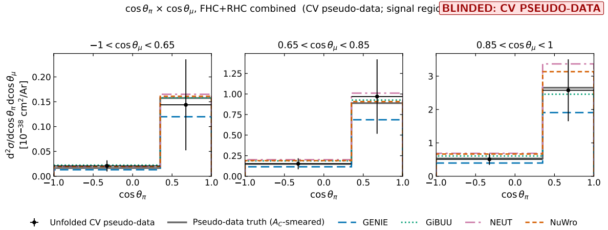
Figure 27: d^2\sigma/d\cos\theta_\pi d\cos\theta_\mu in the combined configuration, as slices in \cos\theta_\mu . Points are the unfolded pseudo-data with the total uncertainty, the grey histogram is the A_C -smeared truth of the pseudo-data and the coloured histograms are the generator predictions, smeared with A_C . Each slice has its own vertical scale.
